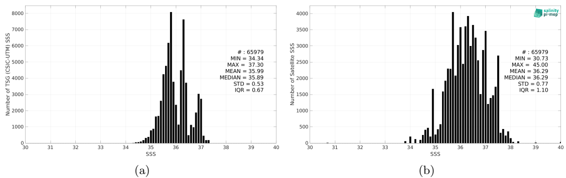
Figure 2: Histograms of SSS from TSG (CSIC-UTM) (a) and SMAP SSS L2 v5.0 (JPL) (b) considering all match-up pairs per bins of 0.1 over the Amazon and Orinoco river plumes Pi-MEP region and for the full satellite product period.
