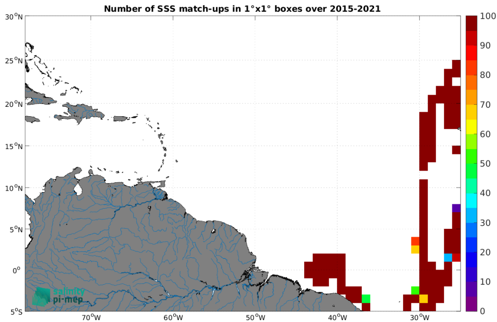
Figure 4: Number of SSS match-ups between TSG (CSIC-UTM) SSS and the SMAP SSS L2 v5.0 (JPL) SSS product for the Amazon and Orinoco river plumes Pi-MEP region over 1^\circ \times 1^\circ boxes and for the full satellite product period.
