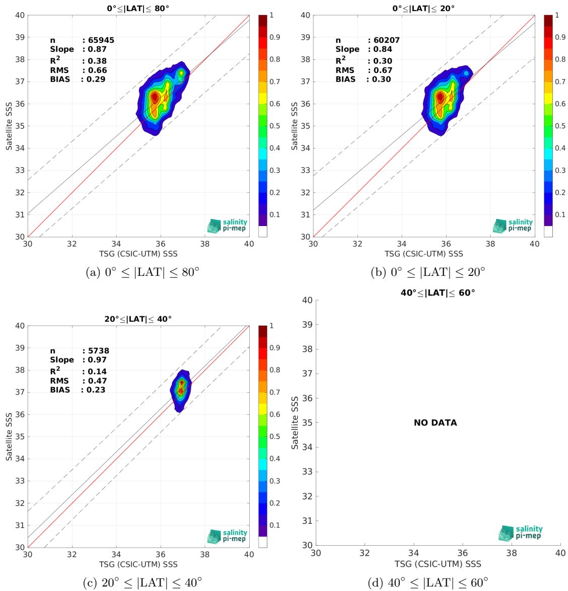
Figure 9: Contour maps of the concentration of SMAP SSS L2 v5.0 (JPL) SSS (y-axis) versus TSG (CSIC-UTM) SSS (x-axis) at match-up pairs for different latitude bands. For each plot, the red line shows x=y . The black thin and dashed lines indicate a linear fit through the data cloud and the \pm 95\% confidence levels, respectively. The number match-up pairs n , the slope and R^2 coefficient of the linear fit, the root mean square (RMS) and the mean bias between satellite and in situ data are indicated for each latitude band in each plots.
