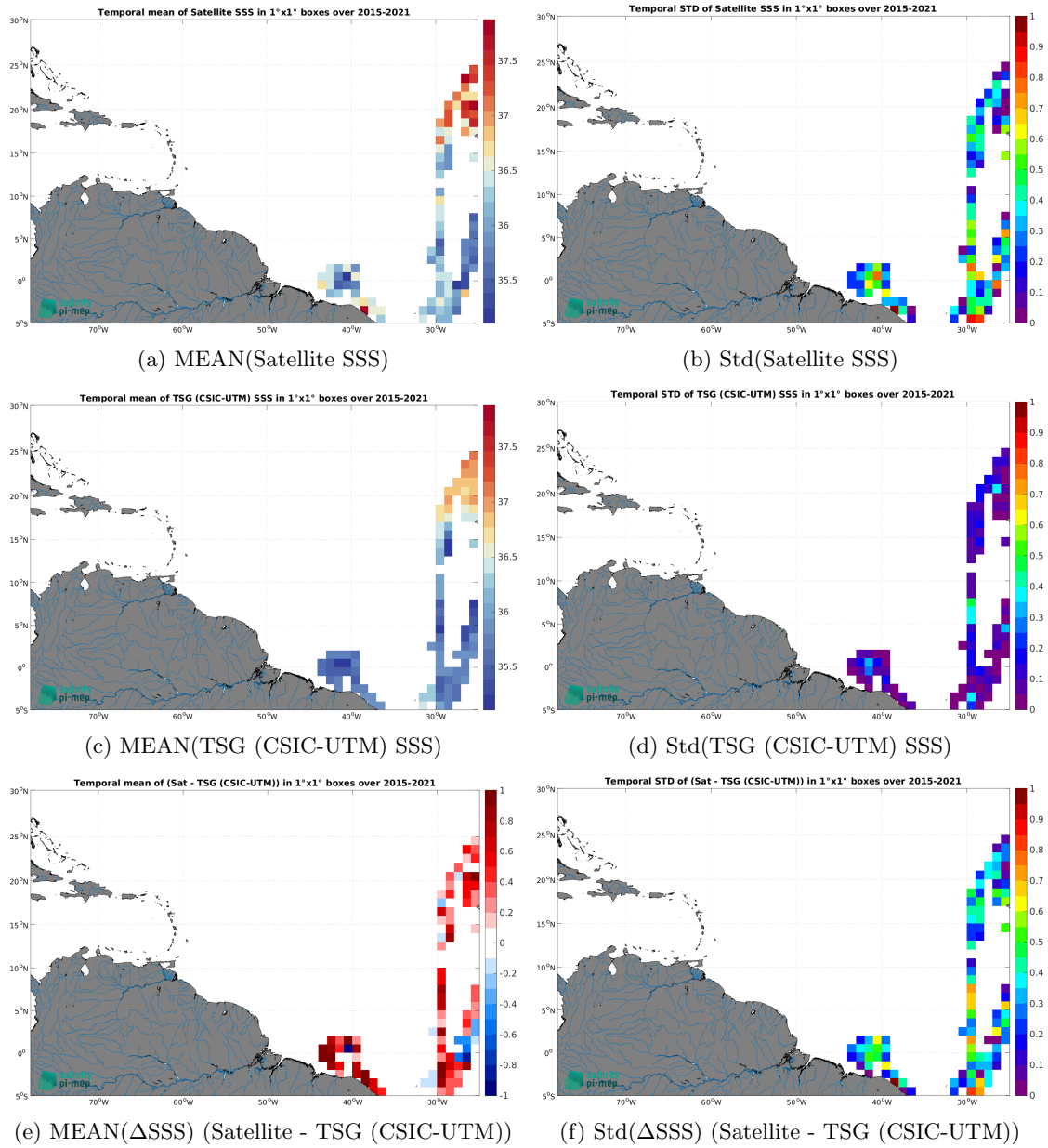
Figure 6: Temporal mean (left) and Std (right) of SSS from SMAP SSS L2 v5.0 (JPL) (top), TSG (CSIC-UTM) (middle), and of \Delta SSS (Satellite - TSG (CSIC-UTM)). Only match-up pairs are used to generate these maps.
