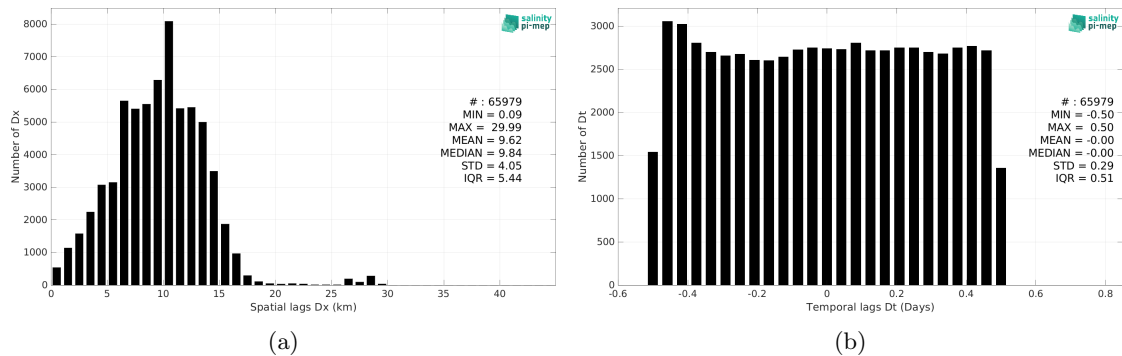
Figure 5: Histograms of the spatial (a) and temporal (b) lags between the location/time of the TSG (CSIC-UTM) measurement and the date of the corresponding SMAP SSS L2 v5.0 (JPL) SSS pixel.
