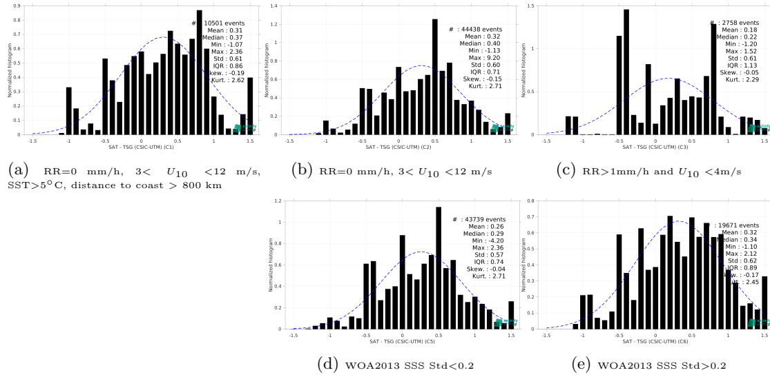
Figure 13: Normalized histogram of \Delta SSS (SMAP SSS L2 v5.0 (JPL) - TSG (CSIC-UTM)) for 5 different subdatasets corresponding to: RR=0 mm/h, 3 < U_{10} < 12 m/s, SST>5°C, distance to coast > 800 km (a), RR=0 mm/h, 3 < U_{10} < 12 m/s (b), RR>1mm/h and U_{10} < 4 m/s (c), WOA2013 SSS Std<0.2 (d), WOA2013 SSS Std>0.2 (e).
