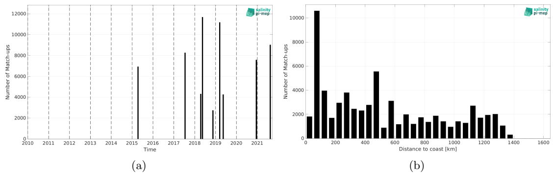
Figure 1: Number of match-ups between TSG (CSIC-UTM) and SMAP SSS L2 v5.0 (JPL) SSS as a function of time (a) and as function of the distance to coast (b) over the Amazon and Orinoco river plumes Pi-MEP region and for the full satellite product period.
