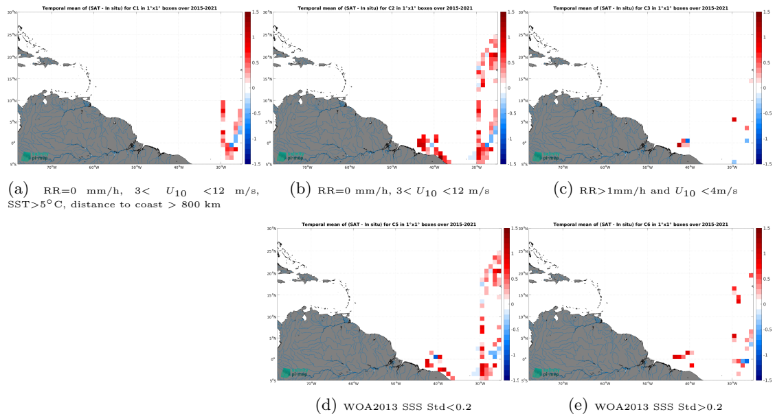
Figure 12: Temporal mean gridded over spatial boxes of size 1^\circ \times 1^\circ of \Delta SSS (SMAP SSS L2 v5.0 (JPL) - TSG (CSIC-UTM)) for 5 different subdatasets corresponding to:RR=0 mm/h, 3 < U_{10} < 12 m/s, SST > 5^\circ\text{C} , distance to coast > 800 km (a), RR=0 mm/h, 3 < U_{10} < 12 m/s (b), RR > 1 mm/h and U_{10} < 4 m/s (c), WOA2013 SSS Std < 0.2 (d), WOA2013 SSS Std > 0.2 (e).
