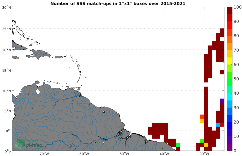
Figure 4: Number of SSS match-ups between TSG (CSIC-UTM) SSS and the SMAP SSS L2 v5.0 (JPL) SSS product for the Amazon and Orinoco river plumes Pi-MEP region over 1°x1° boxes and for the full satellite product period.
