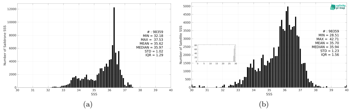
Figure 3: Histograms of SSS from Sairdrone (a) and SMAP SSS L2 v5.0 (JPL) (b) considering all match-up pairs per bins of 0.1 over the Amazon and Orinoco river plumes Pi-MEP region and for the full satellite product period.
