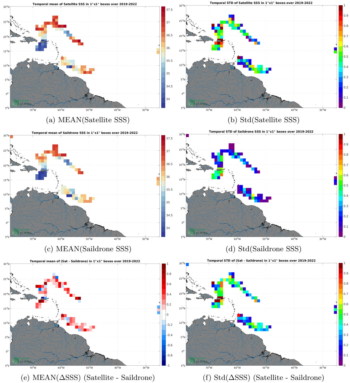
Figure 6: Temporal mean (left) and Std (right) of SSS from SMAP SSS L2 v5.0 (JPL) (top), Saildrone (middle), and of \Delta SSS (Satellite - Saildrone). Only match-up pairs are used to generate these maps.
