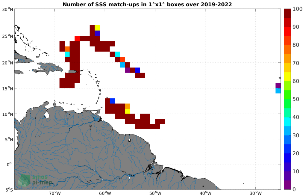
Figure 4: Number of SSS match-ups between Saildrone SSS and the SMAP SSS L2 v5.0 (JPL) SSS product for the Amazon and Orinoco river plumes Pi-MEP region over 1°×1° boxes and for the full satellite product period.
