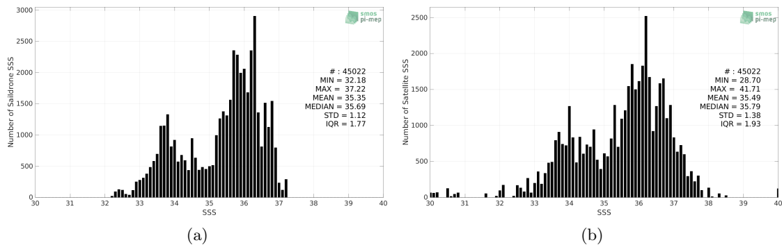
Figure 2: Histograms of SSS from Saildrone (a) and SMAP SSS L2 v5.0 (JPL) (b) considering all match-up pairs per bins of 0.1 over the Amazon and Orinoco river plumes Pi-MEP region and for the full satellite product period.
