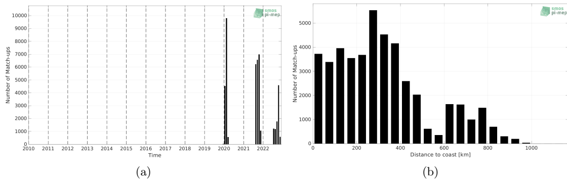
Figure 1: Number of match-ups between Saildrone and SMAP SSS L2 v5.0 (JPL) SSS as a function of time (a) and as function of the distance to coast (b) over the Amazon and Orinoco river plumes Pi-MEP region and for the full satellite product period.
