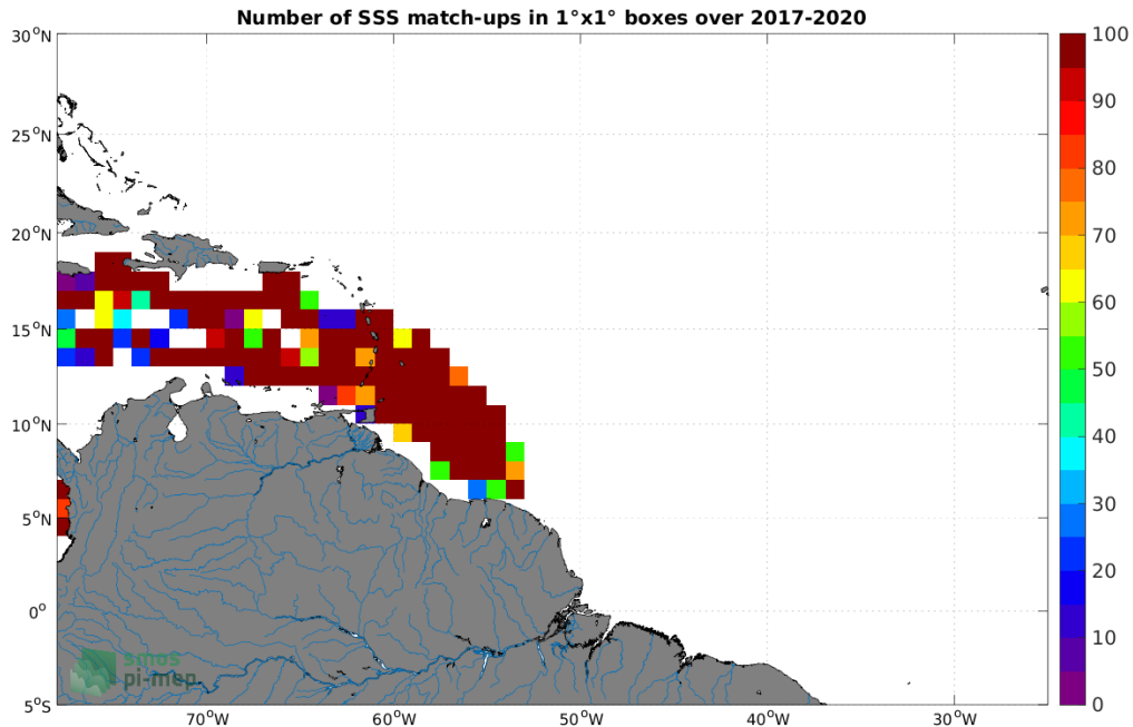
Figure 3: Number of SSS match-ups between Surface drifters SSS and the SMAP SSS L2 v5.0 (JPL) SSS product for the Amazon and Orinoco river plumes Pi-MEP region over 1^\circ \times 1^\circ boxes and for the full satellite product period.
