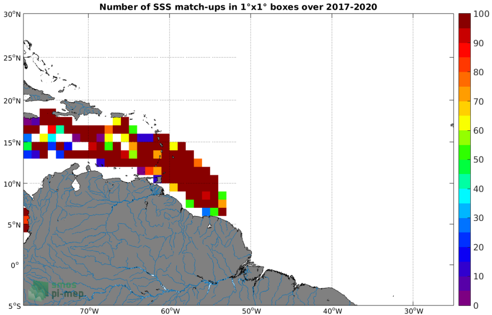
Figure 3: Number of SSS match-ups between Surface drifters SSS and the SMAP SSS L2 v5.0 (JPL) SSS product for the Amazon and Orinoco river plumes Pi-MEP region over 1°x1° boxes and for the full satellite product period.
