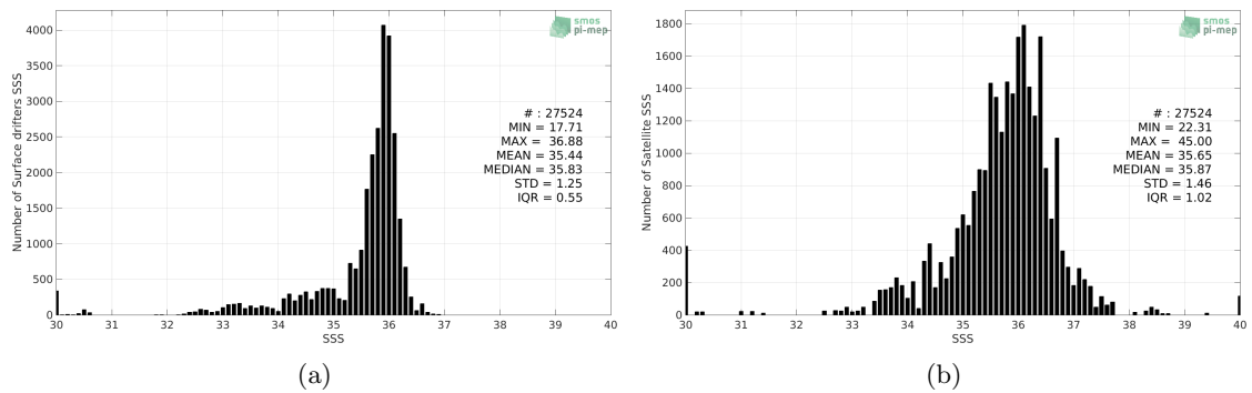
Figure 2: Histograms of SSS from Surface drifters (a) and SMAP SSS L2 v5.0 (JPL) (b) considering all match-up pairs per bins of 0.1 over the Amazon and Orinoco river plumes Pi-MEP region and for the full satellite product period.
