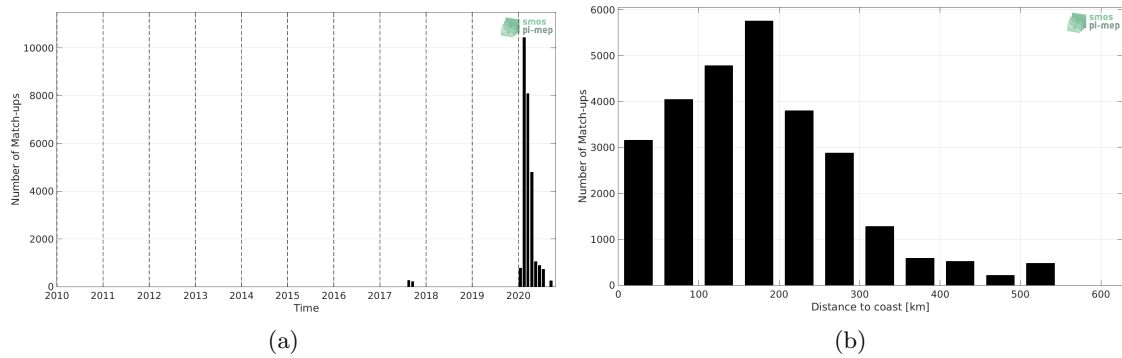
Figure 1: Number of match-ups between Surface drifters and SMAP SSS L2 v5.0 (JPL) SSS as a function of time (a) and as function of the distance to coast (b) over the Amazon and Orinoco river plumes Pi-MEP region and for the full satellite product period.
