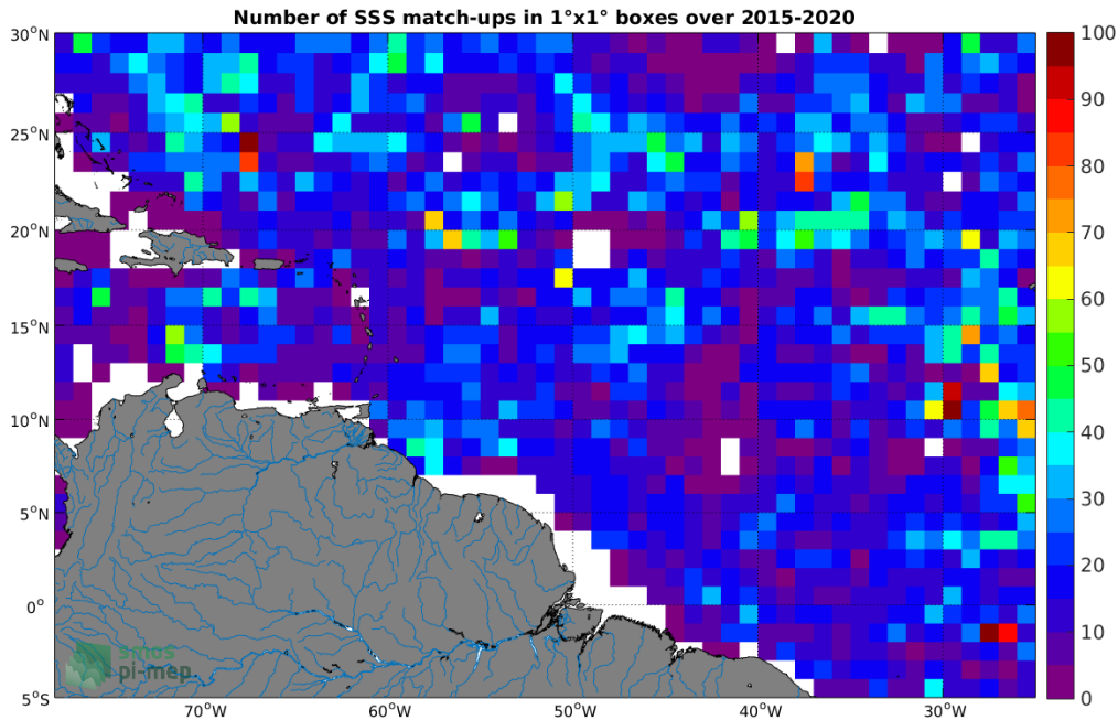
Figure 4: Number of SSS match-ups between Argo SSS and the SMAP SSS L2 v5.0 (JPL) SSS product for the Amazon and Orinoco river plumes Pi-MEP region over 1°x1° boxes and for the full satellite product period.
