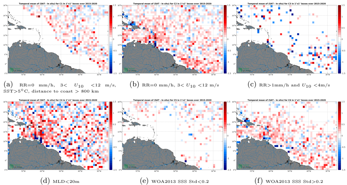
Figure 12: Temporal mean gridded over spatial boxes of size 1°x1° of \Delta SSS (SMAP SSS L2 v5.0 (JPL) - Argo) for 6 different subdatasets corresponding to:RR=0 mm/h, 3 < U_{10} < 12 m/s, SST>5°C, distance to coast > 800 km (a), RR=0 mm/h, 3 < U_{10} < 12 m/s (b), RR>1mm/h and U_{10} < 4 m/s (c),MLD<20m (d),WOA2013 SSS Std<0.2 (e),WOA2013 SSS Std>0.2 (f).
