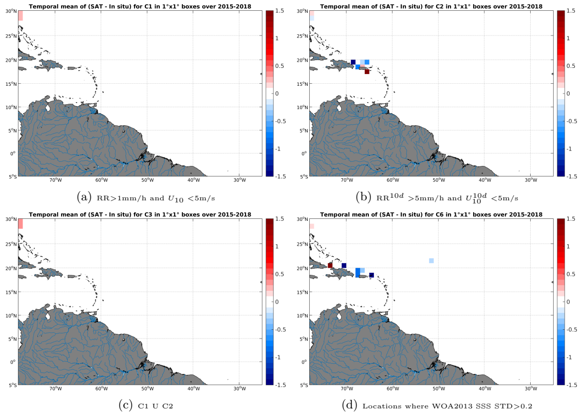
Figure 12: Temporal mean gridded over spatial boxes of size 1^\circ \times 1^\circ of \Delta SSS (SMAP-L2-JPL-V4 - TSG-SAMOS) for 4 different subdatasets corresponding to: RR > 1\text{mm/h} and U_{10} < 5\text{m/s} (a), RR^{10d} > 5\text{mm/h} and U_{10}^{10d} < 5\text{m/s} (b), C1 U C2 (c), Locations where WOA2013 SSS STD > 0.2 (d).
