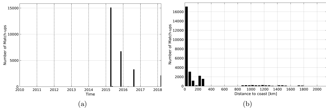
Figure 1: Number of match-ups between TSG-SAMOS and SMAP-L2-JPL-V4 SSS as a function of time (a) and as function of the distance to coast (b) over the Amazon and Orinoco river plumes Pi-MEP region and for the full satellite product period.
