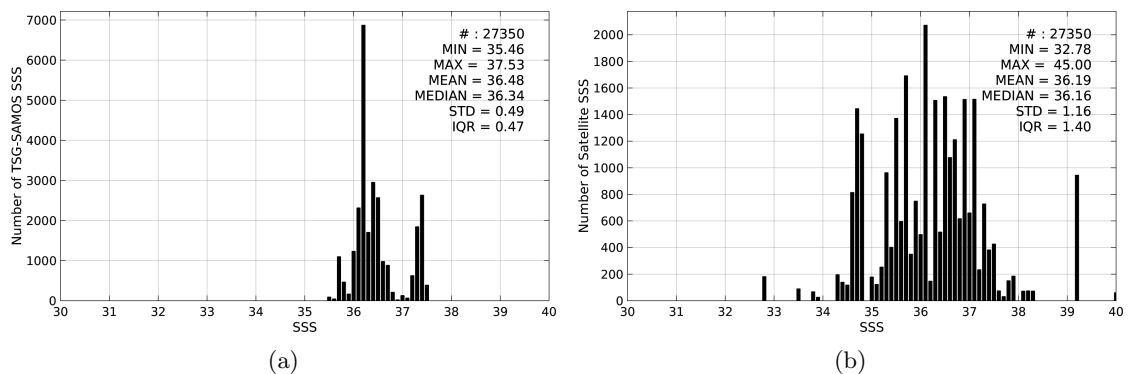
Figure 2: Histograms of SSS from TSG-SAMOS (a) and SMAP-L2-JPL-V4 (b) considering all match-up pairs per bins of 0.1 over the Amazon and Orinoco river plumes Pi-MEP region and for the full satellite product period.
