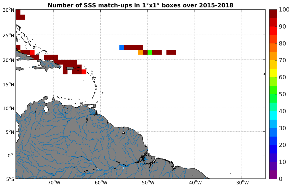
Figure 4: Number of SSS match-ups between TSG-SAMOS SSS and the SMAP-L2-JPL-V4 SSS product for the Amazon and Orinoco river plumes Pi-MEP region over 1^\circ \times 1^\circ boxes and for the full satellite product period.
