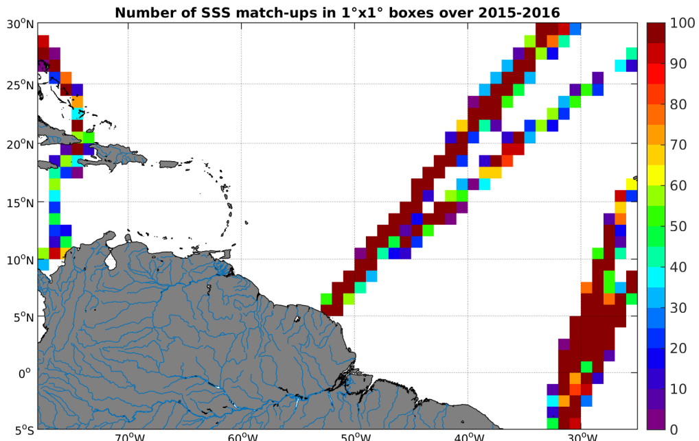
Figure 4: Number of SSS match-ups between TSG-LEGOS-DM SSS and the SMAP-L2-JPL-V4 SSS product for the Amazon and Orinoco river plumes Pi-MEP region over 1^\circ \times 1^\circ boxes and for the full satellite product period.
