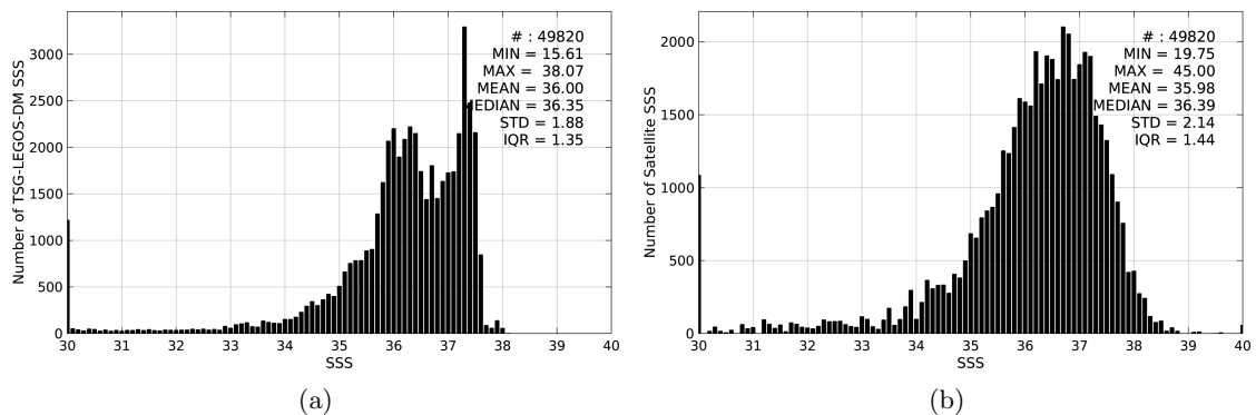
Figure 2: Histograms of SSS from TSG-LEGOS-DM (a) and SMAP-L2-JPL-V4 (b) considering all match-up pairs per bins of 0.1 over the Amazon and Orinoco river plumes Pi-MEP region and for the full satellite product period.
