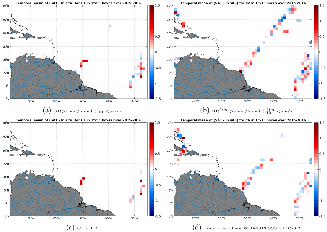
Figure 12: Temporal mean gridded over spatial boxes of size 1^\circ \times 1^\circ of \Delta SSS (SMAP-L2-JPL-V4 - TSG-LEGOS-DM) for 4 different subdatasets corresponding to: RR > 1\text{mm/h} and U_{10} < 5\text{m/s} (a), RR^{10d} > 5\text{mm/h} and U_{10}^{10d} < 5\text{m/s} (b), C1 U C2 (c), Locations where WOA2013 SSS STD > 0.2 (d).
