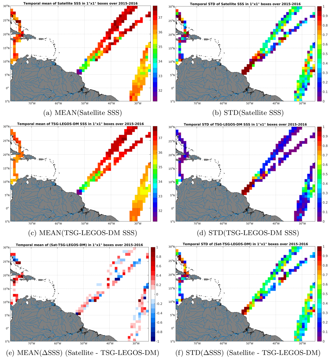
Figure 6: Temporal mean (left) and STD (right) of SSS from SMAP-L2-JPL-V4 (top), TSG-LEGOS-DM (middle), and of \Delta SSS (Satellite - TSG-LEGOS-DM). Only match-up pairs are used to generate these maps.
