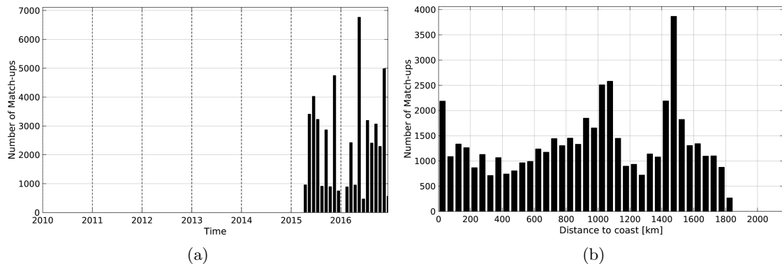
Figure 1: Number of match-ups between TSG-LEGOS-DM and SMAP-L2-JPL-V4 SSS as a function of time (a) and as function of the distance to coast (b) over the Amazon and Orinoco river plumes Pi-MEP region and for the full satellite product period.
