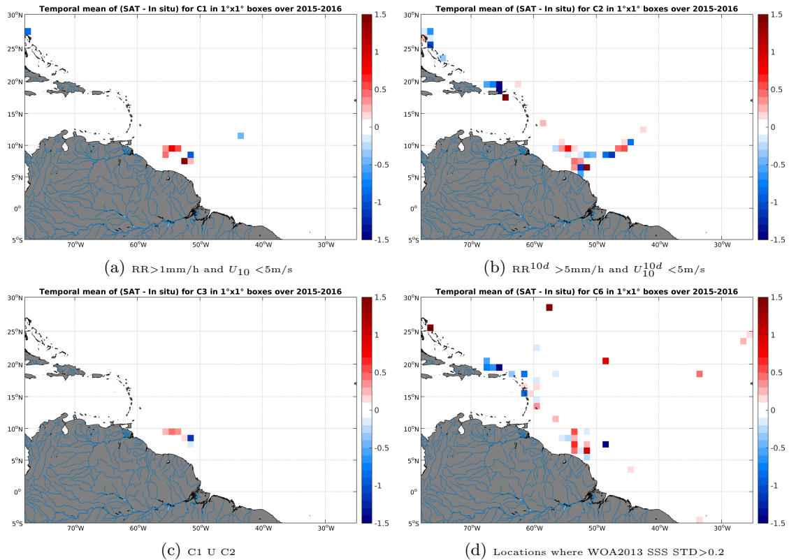
Figure 12: Temporal mean gridded over spatial boxes of size 1°x1° of \Delta SSS (SMAP-L2-JPL-V4 - TSG-GOSUD-Research-vessel) for 4 different subdatasets corresponding to:RR>1mm/h and U_{10} < 5m/s (a), RR^{10d} > 5mm/h and U_{10}^{10d} < 5m/s (b), C1 U C2 (c),Locations where WOA2013 SSS STD>0.2 (d).
