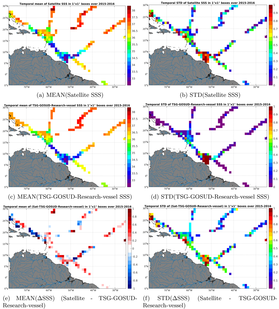
Figure 6: Temporal mean (left) and STD (right) of SSS from SMAP-L2-JPL-V4 (top), TSG-GOSUD-Research-vessel (middle), and of \Delta SSS (Satellite - TSG-GOSUD-Research-vessel). Only match-up pairs are used to generate these maps.
