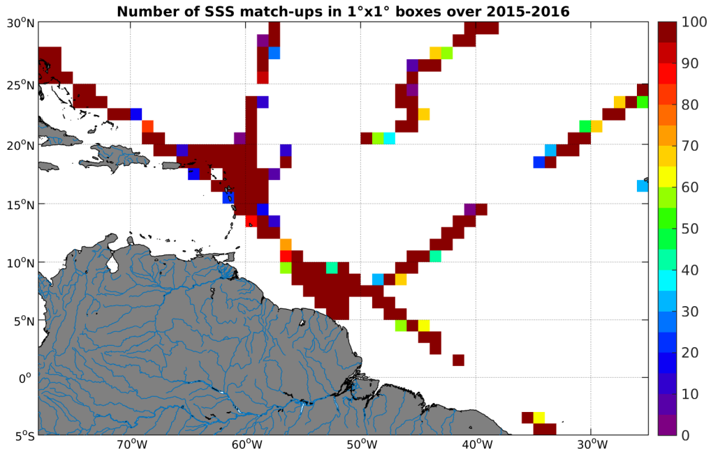
Figure 4: Number of SSS match-ups between TSG-GOSUD-Research-vessel SSS and the SMAP-L2-JPL-V4 SSS product for the Amazon and Orinoco river plumes Pi-MEP region over 1^\circ \times 1^\circ boxes and for the full satellite product period.
