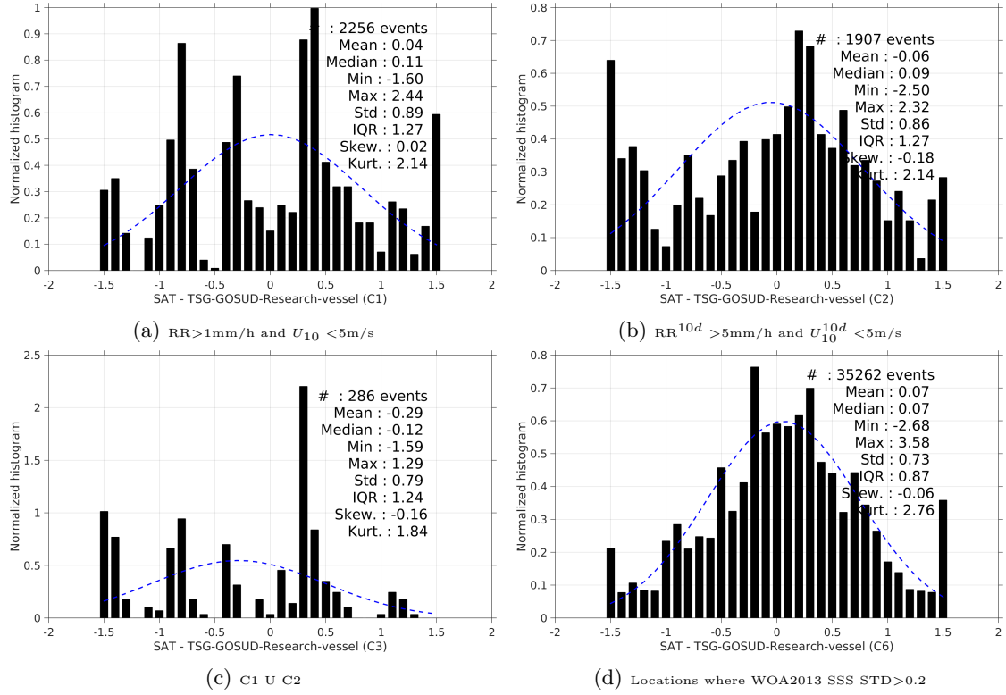
Figure 13: Normalized histogram of \Delta SSS (SMAP-L2-JPL-V4 - TSG-GOSUD-Research-vessel) for 6 different subdatasets corresponding to: RR > 1mm/h and U_{10} < 5\text{m/s} (a), RR^{10d} > 5\text{mm/h} and U_{10}^{10d} < 5\text{m/s} (b), C1 U C2 (c), Locations where WOA2013 SSS STD > 0.2 (d).
