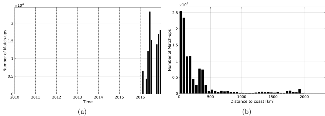
Figure 1: Number of match-ups between TSG-GOSUD-Research-vessel and SMAP-L2-JPL-V4 SSS as a function of time (a) and as function of the distance to coast (b) over the Amazon and Orinoco river plumes Pi-MEP region and for the full satellite product period.
