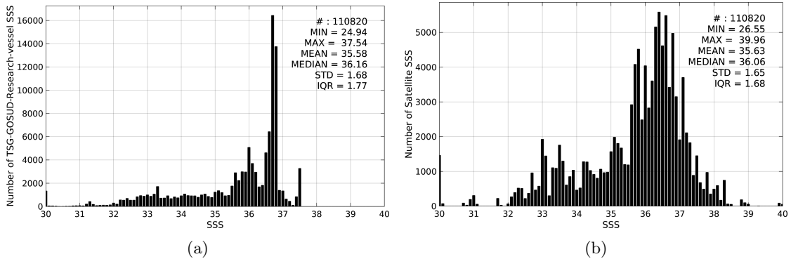
Figure 2: Histograms of SSS from TSG-GOSUD-Research-vessel (a) and SMAP-L2-JPL-V4 (b) considering all match-up pairs per bins of 0.1 over the Amazon and Orinoco river plumes Pi-MEP region and for the full satellite product period.
