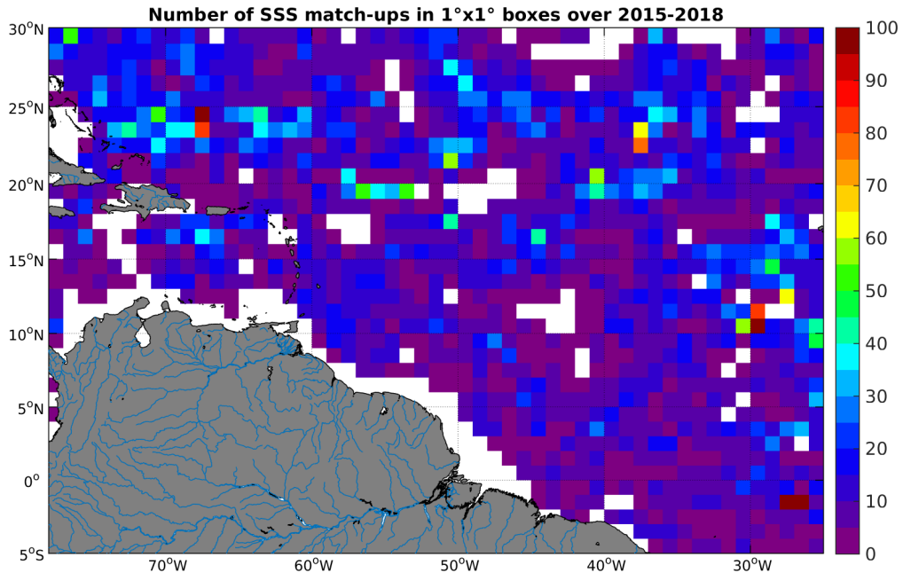
Figure 4: Number of SSS match-ups between Argo SSS and the SMAP-L2-JPL-V4 SSS product for the Amazon and Orinoco river plumes Pi-MEP region over 1°x1° boxes and for the full satellite product period.
