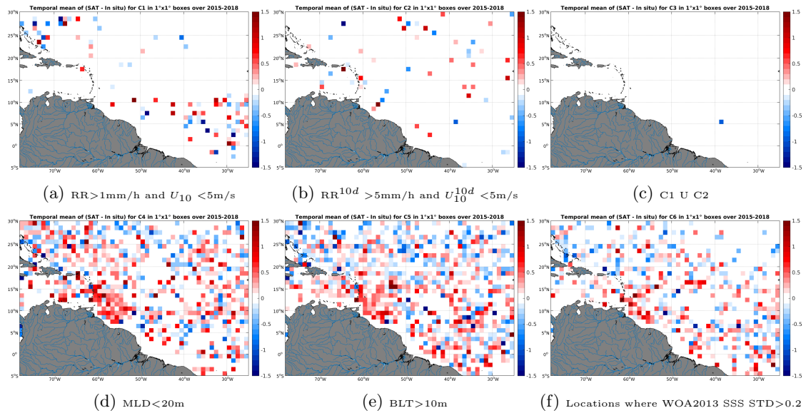
Figure 12: Temporal mean gridded over spatial boxes of size 1^\circ \times 1^\circ of \Delta SSS (SMAP-L2-JPL-V4 - Argo) for 6 different subdatasets corresponding to: RR > 1\text{mm/h} and U_{10} < 5\text{m/s} (a), RR^{10d} > 5\text{mm/h} and U_{10}^{10d} < 5\text{m/s} (b), C1 U C2 (c), MLD < 20\text{m} (d), BLT > 10\text{m} (e), Locations where WOA2013 SSS STD > 0.2 (f).
