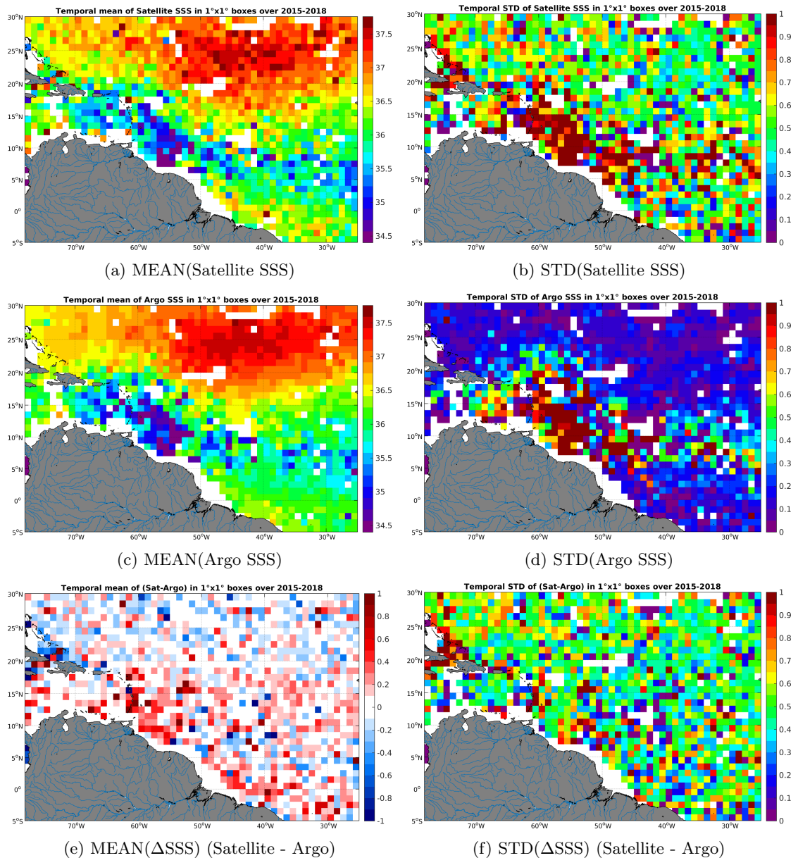
Figure 6: Temporal mean (left) and STD (right) of SSS from SMAP-L2-JPL-V4 (top), Argo (middle), and of \Delta SSS (Satellite - Argo). Only match-up pairs are used to generate these maps.
