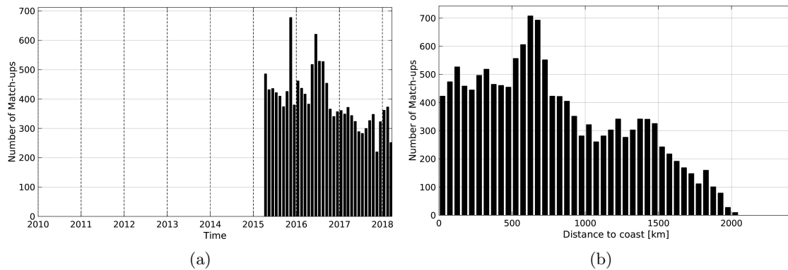
Figure 1: Number of match-ups between Argo and SMAP-L2-JPL-V4 SSS as a function of time (a) and as function of the distance to coast (b) over the Amazon and Orinoco river plumes Pi-MEP region and for the full satellite product period.
