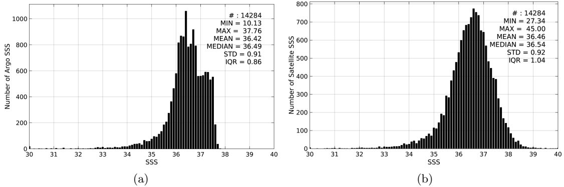
Figure 2: Histograms of SSS from Argo (a) and SMAP-L2-JPL-V4 (b) considering all match-up pairs per bins of 0.1 over the Amazon and Orinoco river plumes Pi-MEP region and for the full satellite product period.
