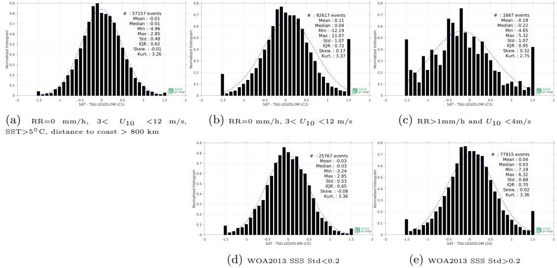
Figure 13: Normalized histogram of \Delta SSS (SMAP-L2-JPL-V4.3 - TSG-LEGOS-DM) for 5 different subdatasets corresponding to: RR=0 mm/h, 3 < U_{10} < 12 m/s, SST>5°C, distance to coast > 800 km (a), RR=0 mm/h, 3 < U_{10} < 12 m/s (b), RR>1mm/h and U_{10} < 4 m/s (c), WOA2013 SSS Std<0.2 (d), WOA2013 SSS Std>0.2 (e).
