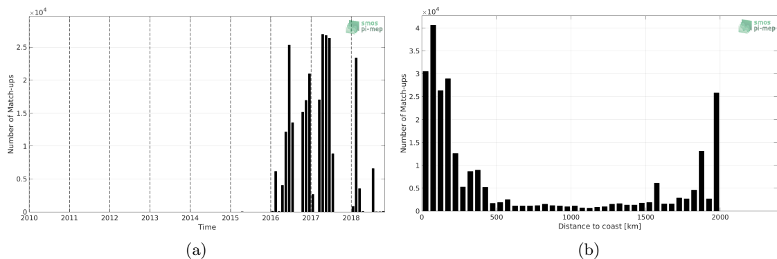
Figure 1: Number of match-ups between TSG-GOSUD-Research-vessel and SMAP-L2-JPL-V4.3 SSS as a function of time (a) and as function of the distance to coast (b) over the Amazon and Orinoco river plumes Pi-MEP region and for the full satellite product period.
