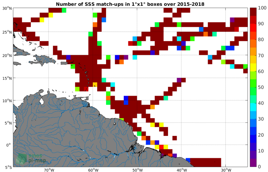
Figure 4: Number of SSS match-ups between TSG-GOSUD-Research-vessel SSS and the SMAP-L2-JPL-V4.3 SSS product for the Amazon and Orinoco river plumes Pi-MEP region over 1^\circ \times 1^\circ boxes and for the full satellite product period.
