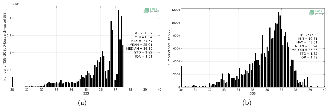
Figure 2: Histograms of SSS from TSG-GOSUD-Research-vessel (a) and SMAP-L2-JPL-V4.3 (b) considering all match-up pairs per bins of 0.1 over the Amazon and Orinoco river plumes Pi-MEP region and for the full satellite product period.
