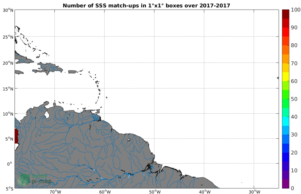
Figure 3: Number of SSS match-ups between Surface drifters SSS and the SMAP-L2-JPL-V4.3 SSS product for the Amazon and Orinoco river plumes Pi-MEP region over 1^{\circ} \times 1^{\circ} boxes and for the full satellite product period.
