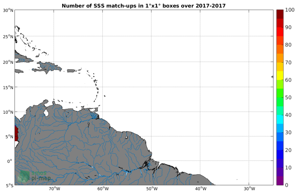
Figure 3: Number of SSS match-ups between Surface drifters SSS and the SMAP-L2-JPL-V4.3 SSS product for the Amazon and Orinoco river plumes Pi-MEP region over 1^\circ \times 1^\circ boxes and for the full satellite product period.
