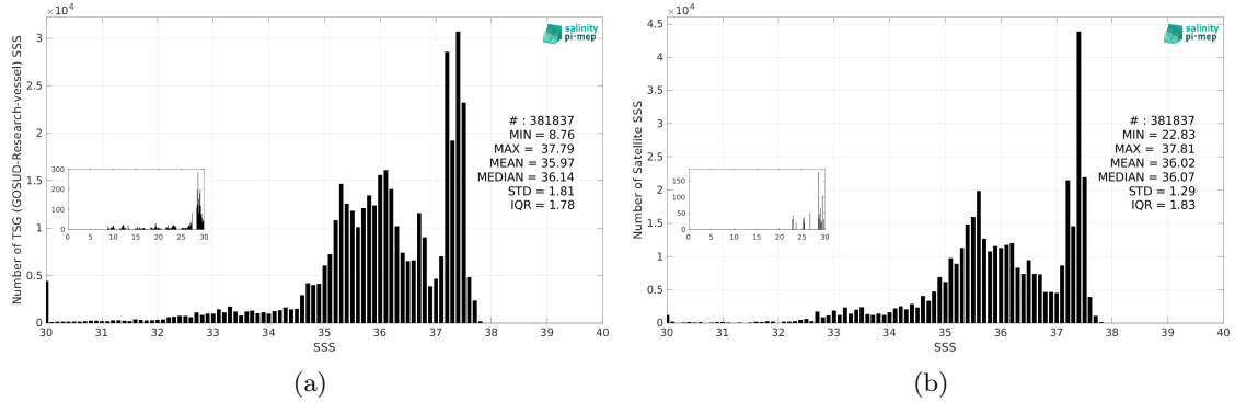
Figure 3: Histograms of SSS from TSG (GOSUD-Research-vessel) (a) and CCI SSS L4 Merged-OI v4.41 - 7-day running (ESA) (b) considering all match-up pairs per bins of 0.1 over the Amazon and Orinoco river plumes Pi-MEP region and for the full satellite product period.
