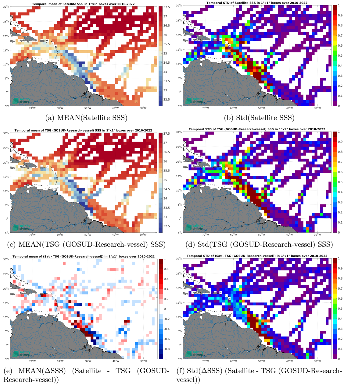
Figure 7: Temporal mean (left) and Std (right) of SSS from CCI SSS L4 Merged-OI v4.41 - 7-day running (ESA) (top), TSG (GOSUD-Research-vessel) (middle), and of \Delta SSS (Satellite - TSG (GOSUD-Research-vessel)). Only match-up pairs are used to generate these maps.
