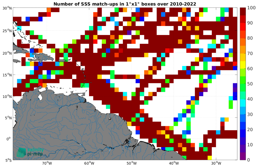
Figure 5: Number of SSS match-ups between TSG (GOSUD-Research-vessel) SSS and the CCI SSS L4 Merged-OI v4.41 - 7-day running (ESA) SSS product for the Amazon and Orinoco river plumes Pi-MEP region over 1^\circ \times 1^\circ boxes and for the full satellite product period.
