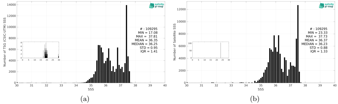
Figure 3: Histograms of SSS from TSG (CSIC-UTM) (a) and CCI SSS L4 Merged-OI v4.41 - 7-day running (ESA) (b) considering all match-up pairs per bins of 0.1 over the Amazon and Orinoco river plumes Pi-MEP region and for the full satellite product period.
