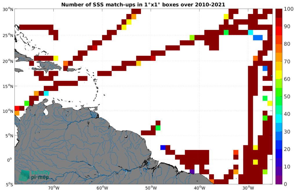
Figure 5: Number of SSS match-ups between TSG (CSIC-UTM) SSS and the CCI SSS L4 Merged-OI v4.41 - 7-day running (ESA) SSS product for the Amazon and Orinoco river plumes Pi-MEP region over 1^\circ \times 1^\circ boxes and for the full satellite product period.
