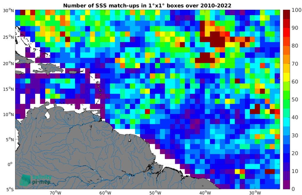
Figure 5: Number of SSS match-ups between Argo SSS and the CCI SSS L4 Merged-OI v4.41 - 7-day running (ESA) SSS product for the Amazon and Orinoco river plumes Pi-MEP region over 1^{\circ} \times 1^{\circ} boxes and for the full satellite product period.
