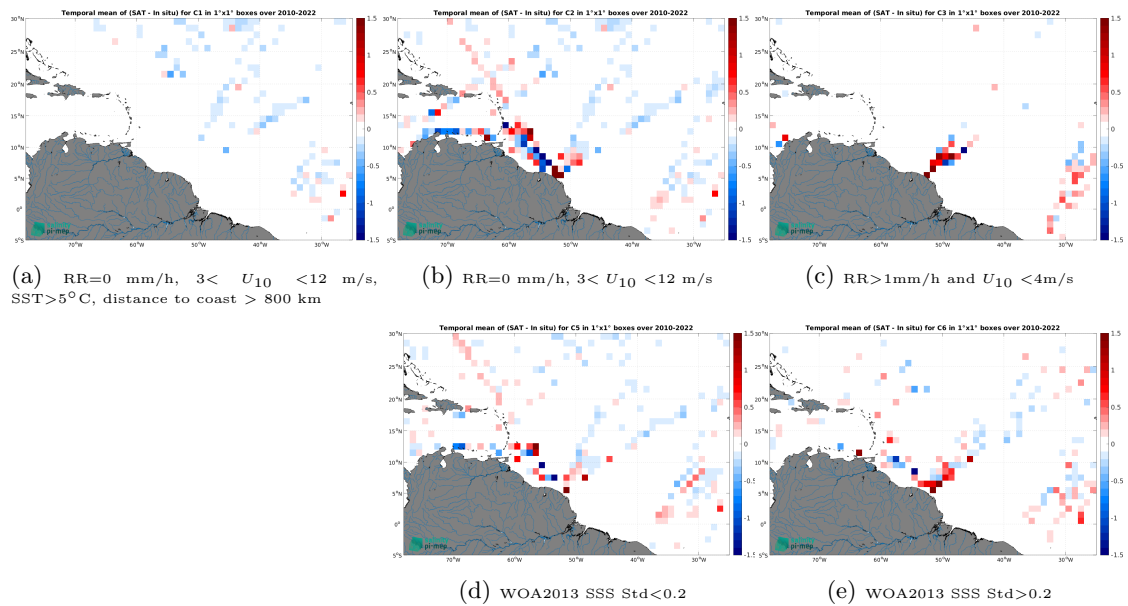
Figure 14: Temporal mean gridded over spatial boxes of size 1^\circ \times 1^\circ of \Delta\text{SSS} (CCI SSS L4 Merged-OI v4.41 - 30-day running (ESA) - TSG (LEGOS-DM)) for 5 different subdatasets corresponding to:RR=0 mm/h, 3 < U_{10} < 12 m/s, SST >5^\circ\text{C} , distance to coast > 800 km (a), RR=0 mm/h, 3 < U_{10} < 12 m/s (b), RR >1 mm/h and U_{10} < 4 m/s (c), WOA2013 SSS Std <0.2 (d), WOA2013 SSS Std >0.2 (e).
