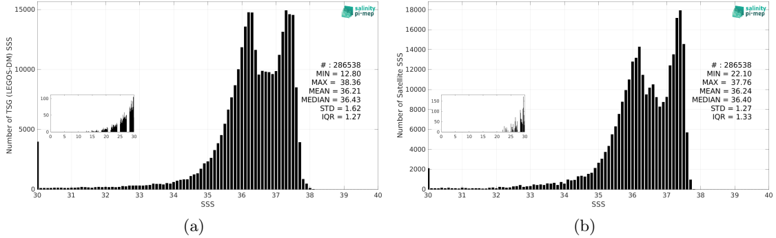
Figure 3: Histograms of SSS from TSG (LEGOS-DM) (a) and CCI SSS L4 Merged-OI v4.41 - 30-day running (ESA) (b) considering all match-up pairs per bins of 0.1 over the Amazon and Orinoco river plumes Pi-MEP region and for the full satellite product period.
