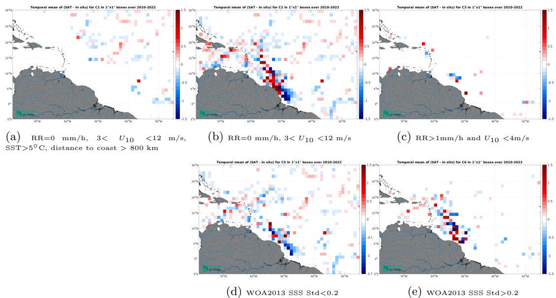
Figure 14: Temporal mean gridded over spatial boxes of size 1^\circ \times 1^\circ of \Delta SSS (CCI SSS L4 Merged-OI v4.41 - 30-day running (ESA) - TSG (GOSUD-Research-vessel)) for 5 different subdatasets corresponding to:RR=0 mm/h, 3 < U_{10} < 12 m/s, SST >5^\circ C, distance to coast > 800 km (a), RR=0 mm/h, 3 < U_{10} < 12 m/s (b), RR >1 mm/h and U_{10} < 4 m/s (c), WOA2013 SSS Std <0.2 (d), WOA2013 SSS Std >0.2 (e).
