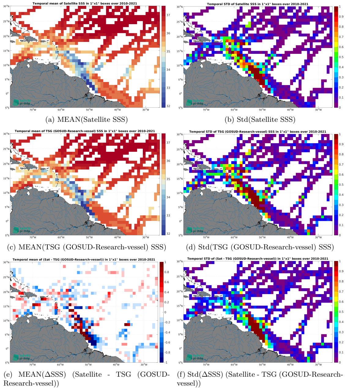
Figure 7: Temporal mean (left) and Std (right) of SSS from CCI SSS L4 Merged-OI v4.41 - 30-day running (ESA) (top), TSG (GOSUD-Research-vessel) (middle), and of \Delta SSS (Satellite - TSG (GOSUD-Research-vessel)). Only match-up pairs are used to generate these maps.
