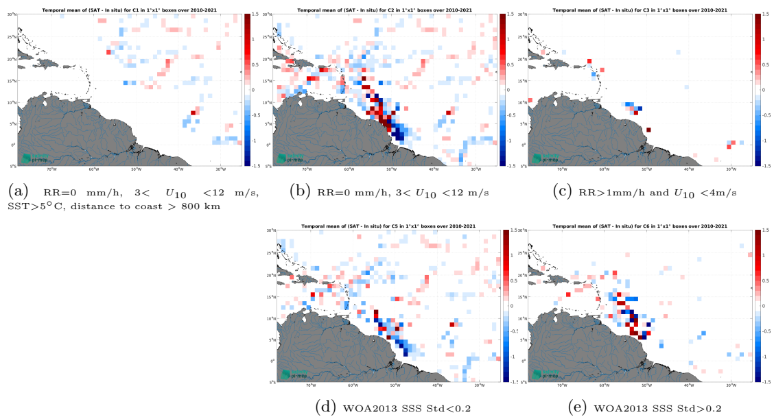
Figure 14: Temporal mean gridded over spatial boxes of size 1^\circ \times 1^\circ of \Delta\text{SSS} (CCI SSS L4 Merged-OI v4.41 - 30-day running (ESA) - TSG (GOSUD-Research-vessel)) for 5 different subdatasets corresponding to:RR=0 mm/h, 3 < U_{10} < 12 m/s, SST >5^\circ\text{C} , distance to coast > 800 km (a), RR=0 mm/h, 3 < U_{10} < 12 m/s (b), RR >1 mm/h and U_{10} < 4 m/s (c), WOA2013 SSS Std <0.2 (d), WOA2013 SSS Std >0.2 (e).
