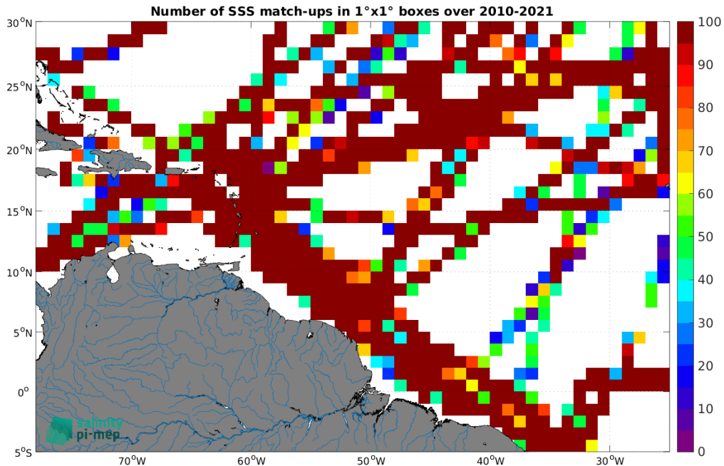
Figure 5: Number of SSS match-ups between TSG (GOSUD-Research-vessel) SSS and the CCI SSS L4 Merged-OI v4.41 - 30-day running (ESA) SSS product for the Amazon and Orinoco river plumes Pi-MEP region over 1^\circ \times 1^\circ boxes and for the full satellite product period.
