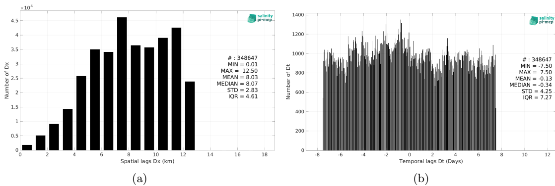
Figure 6: Histograms of the spatial (a) and temporal (b) lags between the location/time of the TSG (GOSUD-Research-vessel) measurement and the date of the corresponding CCI SSS L4 Merged-OI v4.41 - 30-day running (ESA) SSS pixel.
