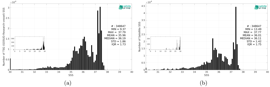
Figure 3: Histograms of SSS from TSG (GOSUD-Research-vessel) (a) and CCI SSS L4 Merged-OI v4.41 - 30-day running (ESA) (b) considering all match-up pairs per bins of 0.1 over the Amazon and Orinoco river plumes Pi-MEP region and for the full satellite product period.
