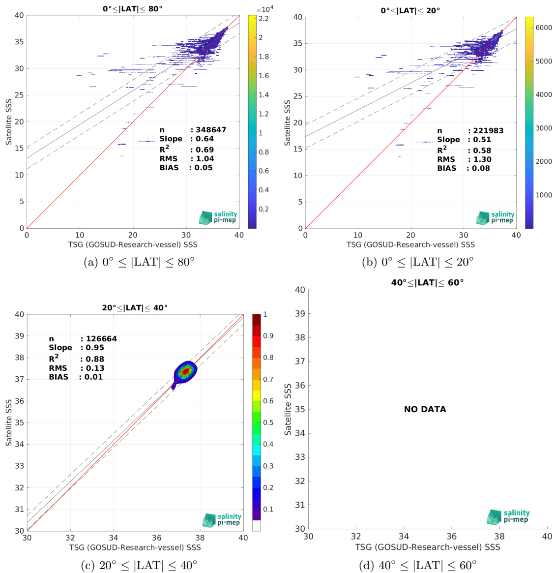
Figure 10: Contour maps of the concentration of CCI SSS L4 Merged-OI v4.41 - 30-day running (ESA) SSS (y-axis) versus TSG (GOSUD-Research-vessel) SSS (x-axis) at match-up pairs for different latitude bands. For each plot, the red line shows x=y . The black thin and dashed lines indicate a linear fit through the data cloud and the \pm 95\% confidence levels, respectively. The number match-up pairs n , the slope and R^2 coefficient of the linear fit, the root mean square (RMS) and the mean bias between satellite and in situ data are indicated for each latitude band in each plots.
