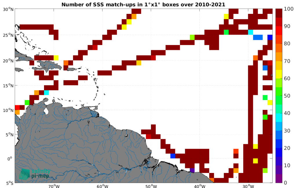
Figure 5: Number of SSS match-ups between TSG (CSIC-UTM) SSS and the CCI SSS L4 Merged-OI v4.41 - 30-day running (ESA) SSS product for the Amazon and Orinoco river plumes Pi-MEP region over 1^\circ \times 1^\circ boxes and for the full satellite product period.
