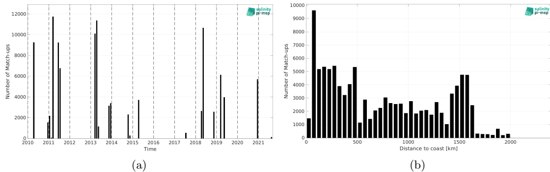
Figure 2: Number of match-ups between TSG (CSIC-UTM) and CCI SSS L4 Merged-OI v4.41 - 30-day running (ESA) SSS as a function of time (a) and as function of the distance to coast (b) over the Amazon and Orinoco river plumes Pi-MEP region and for the full satellite product period.
