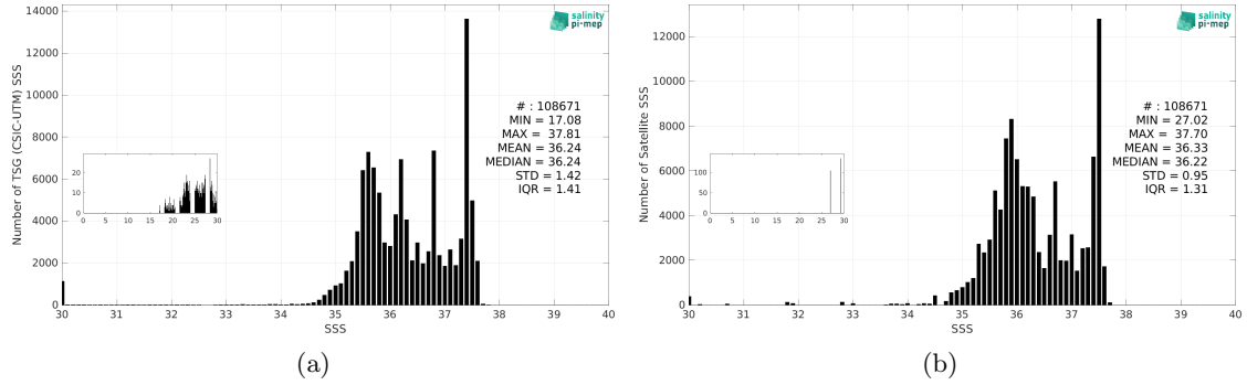
Figure 3: Histograms of SSS from TSG (CSIC-UTM) (a) and CCI SSS L4 Merged-OI v4.41 - 30-day running (ESA) (b) considering all match-up pairs per bins of 0.1 over the Amazon and Orinoco river plumes Pi-MEP region and for the full satellite product period.
