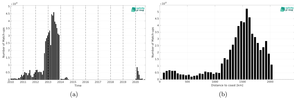
Figure 2: Number of match-ups between Surface drifters and CCI SSS L4 Merged-OI v4.41 - 30-day running (ESA) SSS as a function of time (a) and as function of the distance to coast (b) over the Amazon and Orinoco river plumes Pi-MEP region and for the full satellite product period.
