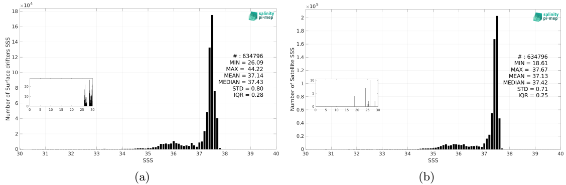
Figure 3: Histograms of SSS from Surface drifters (a) and CCI SSS L4 Merged-OI v4.41 - 30-day running (ESA) (b) considering all match-up pairs per bins of 0.1 over the Amazon and Orinoco river plumes Pi-MEP region and for the full satellite product period.
