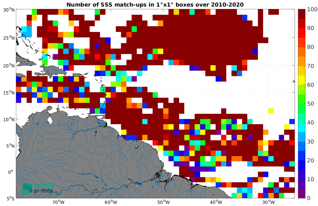
Figure 4: Number of SSS match-ups between Surface drifters SSS and the CCI SSS L4 Merged-OI v4.41 - 30-day running (ESA) SSS product for the Amazon and Orinoco river plumes Pi-MEP region over 1^\circ \times 1^\circ boxes and for the full satellite product period.
