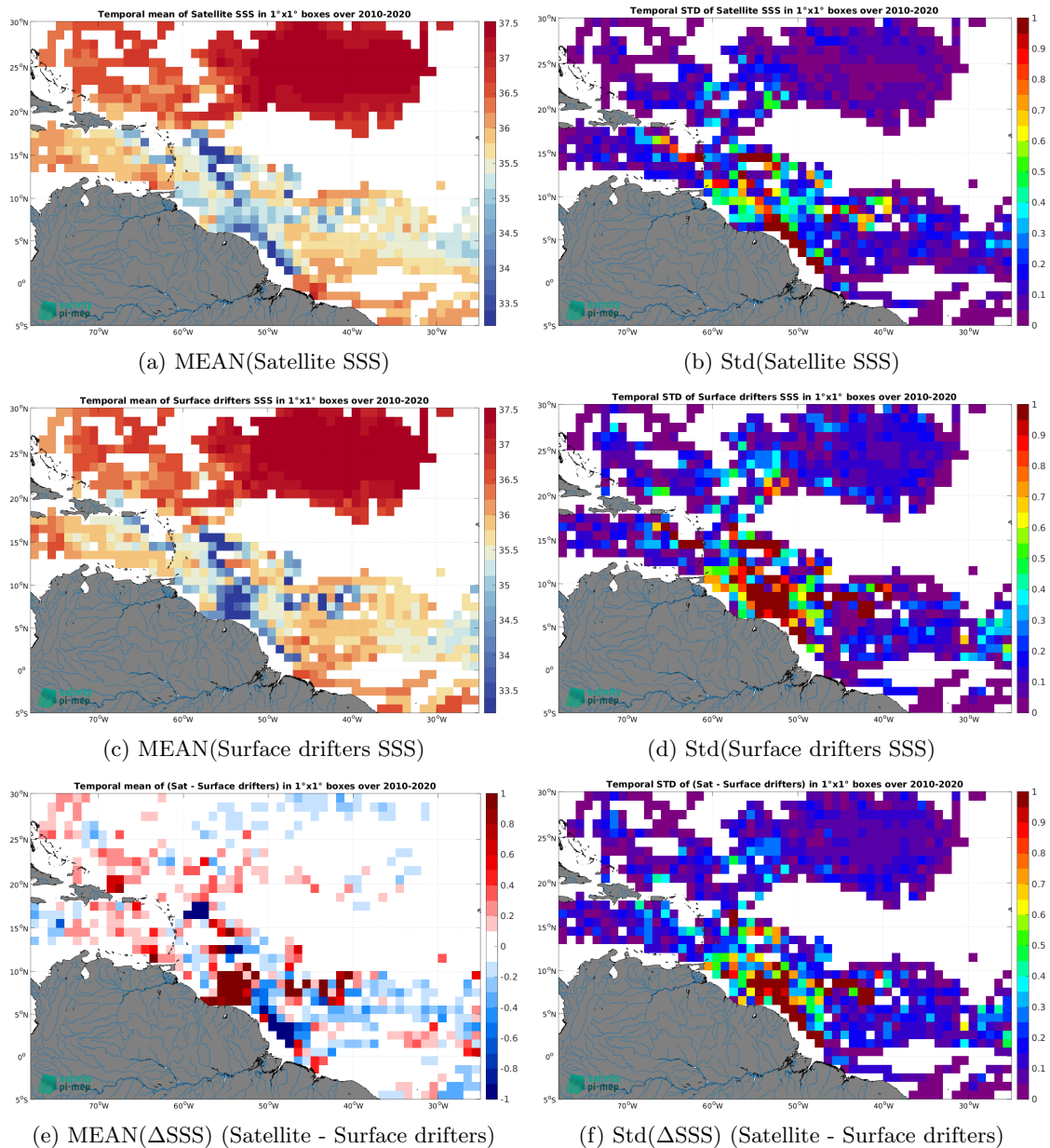
Figure 6: Temporal mean (left) and Std (right) of SSS from CCI SSS L4 Merged-OI v4.41 - 30-day running (ESA) (top), Surface drifters (middle), and of \Delta SSS (Satellite - Surface drifters). Only match-up pairs are used to generate these maps.
