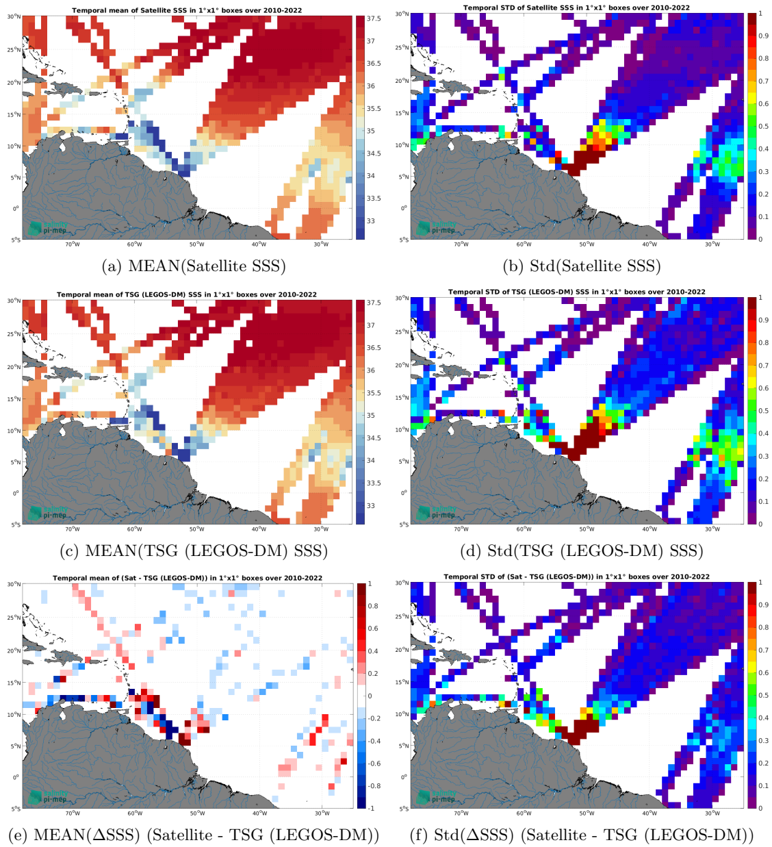
Figure 6: Temporal mean (left) and Std (right) of SSS from CCI SSS L4 Merged-OI v4.4 - 30-day running (ESA) (top), TSG (LEGOS-DM) (middle), and of \Delta SSS (Satellite - TSG (LEGOS-DM)). Only match-up pairs are used to generate these maps.
