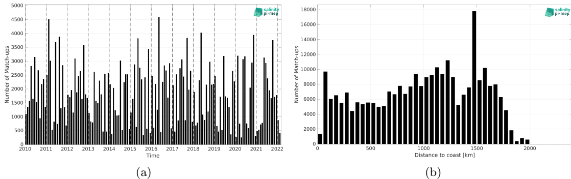
Figure 1: Number of match-ups between TSG (LEGOS-DM) and CCI SSS L4 Merged-OI v4.4 - 30-day running (ESA) SSS as a function of time (a) and as function of the distance to coast (b) over the Amazon and Orinoco river plumes Pi-MEP region and for the full satellite product period.
