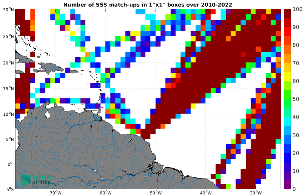
Figure 4: Number of SSS match-ups between TSG (LEGOS-DM) SSS and the CCI SSS L4 Merged-OI v4.4 - 30-day running (ESA) SSS product for the Amazon and Orinoco river plumes Pi-MEP region over 1^\circ \times 1^\circ boxes and for the full satellite product period.
