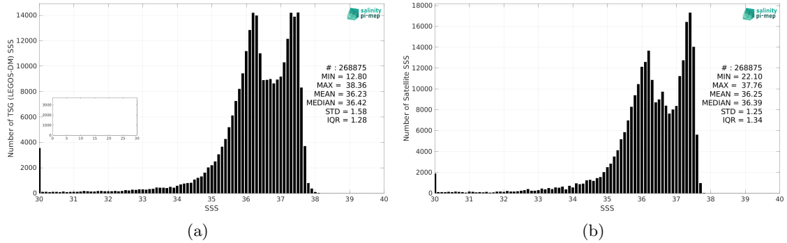
Figure 2: Histograms of SSS from TSG (LEGOS-DM) (a) and CCI SSS L4 Merged-OI v4.4 - 30-day running (ESA) (b) considering all match-up pairs per bins of 0.1 over the Amazon and Orinoco river plumes Pi-MEP region and for the full satellite product period.
