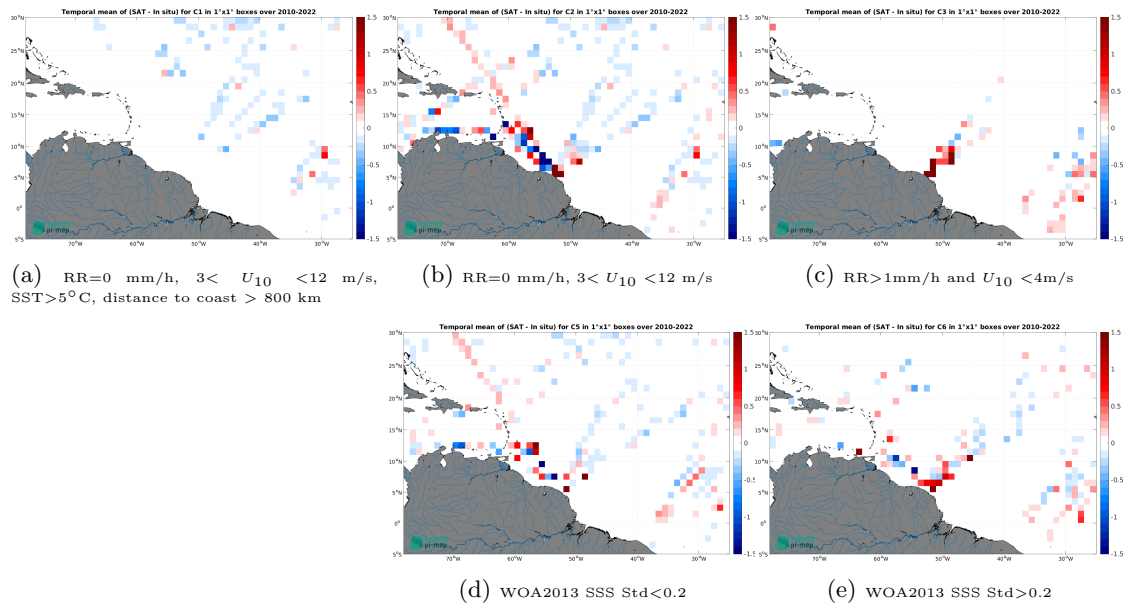
Figure 12: Temporal mean gridded over spatial boxes of size 1^\circ \times 1^\circ of \Delta\text{SSS} (CCI SSS L4 Merged-OI v4.4 - 30-day running (ESA) - TSG (LEGOS-DM)) for 5 different subdatasets corresponding to:RR=0 mm/h, 3 < U_{10} < 12 m/s, SST >5^\circ\text{C} , distance to coast > 800 km (a), RR=0 mm/h, 3 < U_{10} < 12 m/s (b), RR >1 mm/h and U_{10} < 4 m/s (c), WOA2013 SSS Std <0.2 (d), WOA2013 SSS Std >0.2 (e).
