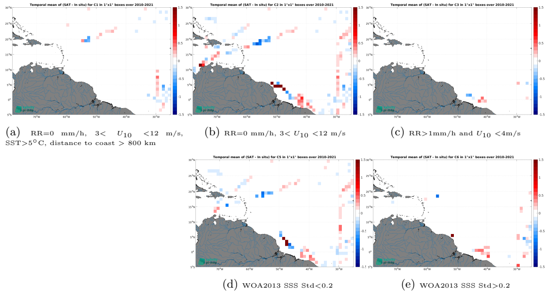
Figure 12: Temporal mean gridded over spatial boxes of size 1^\circ \times 1^\circ of \Delta SSS (CCI SSS L4 Merged-OI v4.4 - 30-day running (ESA) - TSG (CSIC-UTM)) for 5 different subdatasets corresponding to:RR=0 mm/h, 3 < U_{10} < 12 m/s, SST >5^\circ\text{C} , distance to coast > 800 km (a), RR=0 mm/h, 3 < U_{10} < 12 m/s (b), RR >1 mm/h and U_{10} < 4 m/s (c), WOA2013 SSS Std <0.2 (d), WOA2013 SSS Std >0.2 (e).
