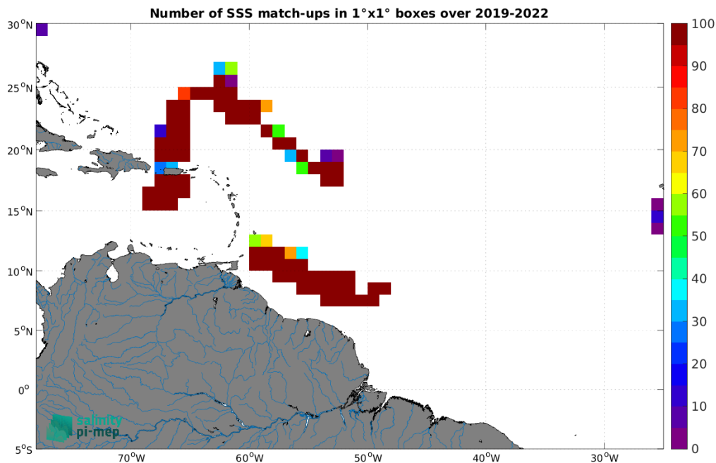
Figure 4: Number of SSS match-ups between Saildrone SSS and the CCI SSS L4 Merged-OI v4.4 - 30-day running (ESA) SSS product for the Amazon and Orinoco river plumes Pi-MEP region over 1^\circ \times 1^\circ boxes and for the full satellite product period.
