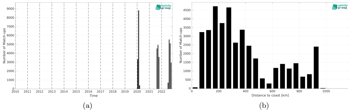
Figure 1: Number of match-ups between Saildrone and CCI SSS L4 Merged-OI v4.4 - 30-day running (ESA) SSS as a function of time (a) and as function of the distance to coast (b) over the Amazon and Orinoco river plumes Pi-MEP region and for the full satellite product period.
