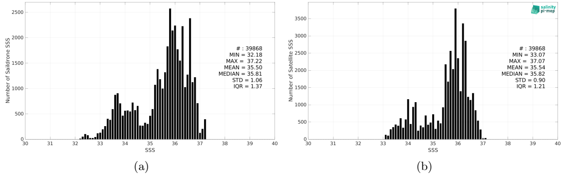
Figure 2: Histograms of SSS from Saildrone (a) and CCI SSS L4 Merged-OI v4.4 - 30-day running (ESA) (b) considering all match-up pairs per bins of 0.1 over the Amazon and Orinoco river plumes Pi-MEP region and for the full satellite product period.
