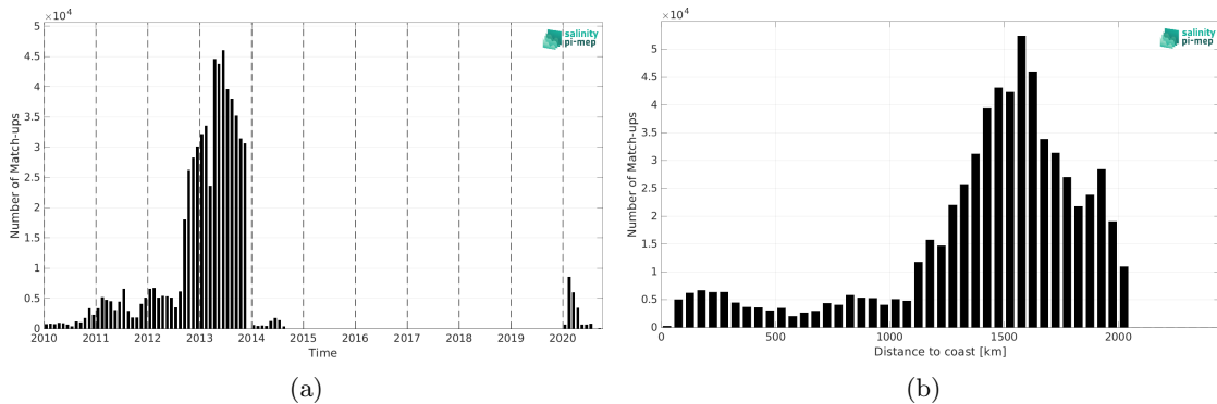
Figure 1: Number of match-ups between Surface drifters and CCI SSS L4 Merged-OI v4.4 - 30-day running (ESA) SSS as a function of time (a) and as function of the distance to coast (b) over the Amazon and Orinoco river plumes Pi-MEP region and for the full satellite product period.
