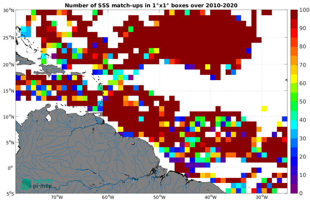
Figure 3: Number of SSS match-ups between Surface drifters SSS and the CCI SSS L4 Merged-OI v4.4 - 30-day running (ESA) SSS product for the Amazon and Orinoco river plumes Pi-MEP region over 1^{\circ} \times 1^{\circ} boxes and for the full satellite product period.
