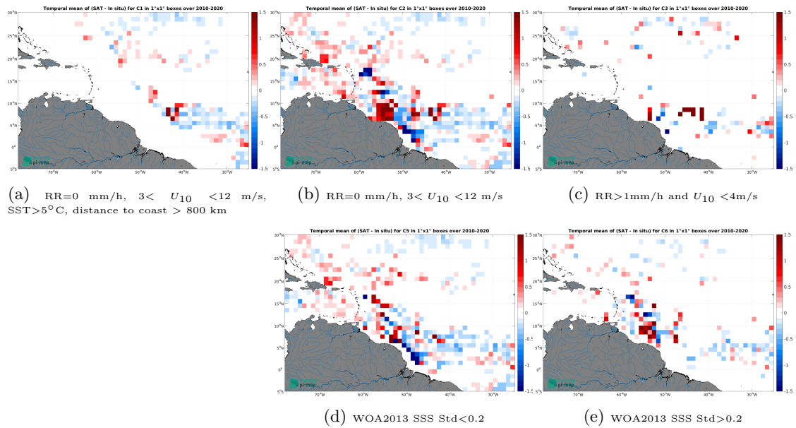
Figure 11: Temporal mean gridded over spatial boxes of size 1^\circ \times 1^\circ of \Delta\text{SSS} (CCI SSS L4 Merged-OI v4.4 - 30-day running (ESA) - Surface drifters) for 5 different subdatasets corresponding to:RR=0 mm/h, 3 < U_{10} < 12 m/s, SST >5^\circ\text{C} , distance to coast > 800 km (a), RR=0 mm/h, 3 < U_{10} < 12 m/s (b), RR >1 mm/h and U_{10} < 4 m/s (c), WOA2013 SSS Std <0.2 (d), WOA2013 SSS Std >0.2 (e).
