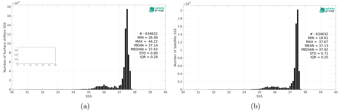
Figure 2: Histograms of SSS from Surface drifters (a) and CCI SSS L4 Merged-OI v4.4 - 30-day running (ESA) (b) considering all match-up pairs per bins of 0.1 over the Amazon and Orinoco river plumes Pi-MEP region and for the full satellite product period.
