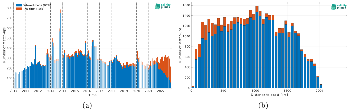
Figure 1: Number of match-ups between Argo and CCI SSS L4 Merged-OI v4.4 - 30-day running (ESA) SSS as a function of time (a) and as function of the distance to coast (b) over the Amazon and Orinoco river plumes Pi-MEP region and for the full satellite product period.
