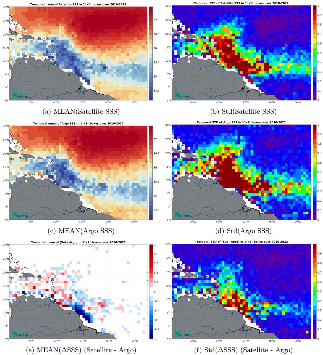
Figure 6: Temporal mean (left) and Std (right) of SSS from CCI SSS L4 Merged-OI v4.4 - 30-day running (ESA) (top), Argo (middle), and of \Delta SSS (Satellite - Argo). Only match-up pairs are used to generate these maps.
