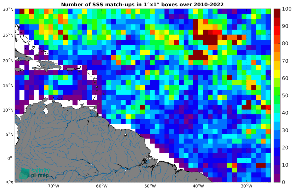
Figure 4: Number of SSS match-ups between Argo SSS and the CCI SSS L4 Merged-OI v4.4 - 30-day running (ESA) SSS product for the Amazon and Orinoco river plumes Pi-MEP region over 1^{\circ} \times 1^{\circ} boxes and for the full satellite product period.
