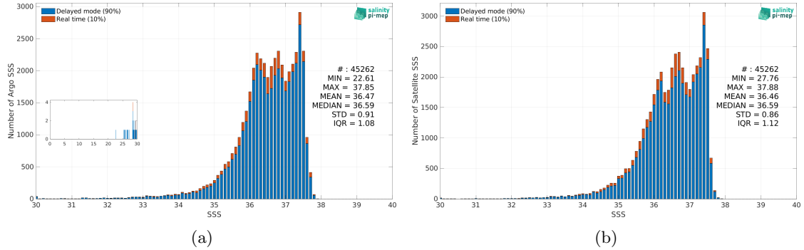
Figure 2: Histograms of SSS from Argo (a) and CCI SSS L4 Merged-OI v4.4 - 30-day running (ESA) (b) considering all match-up pairs per bins of 0.1 over the Amazon and Orinoco river plumes Pi-MEP region and for the full satellite product period.
