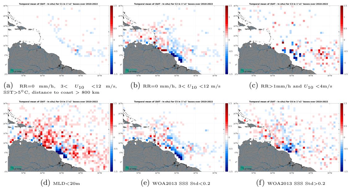
Figure 12: Temporal mean gridded over spatial boxes of size 1^\circ \times 1^\circ of \Delta SSS (CCI SSS L4 Merged-OI v4.4 - 30-day running (ESA) - Argo) for 6 different subdatasets corresponding to:RR=0 mm/h, 3 < U_{10} < 12 m/s, SST >5^\circ C, distance to coast > 800 km (a), RR=0 mm/h, 3 < U_{10} < 12 m/s (b), RR >1 mm/h and U_{10} < 4 m/s (c),MLD <20 m (d),WOA2013 SSS Std <0.2 (e),WOA2013 SSS Std >0.2 (f).
