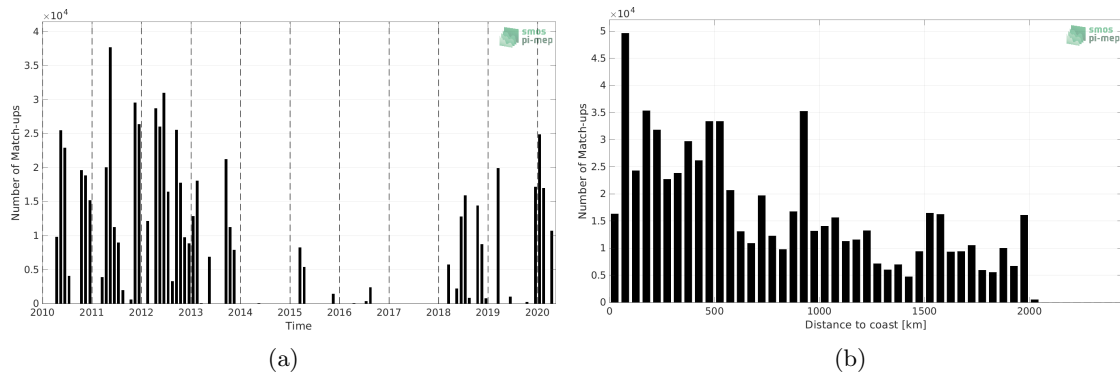
Figure 1: Number of match-ups between TSG (SAMOS) and CCI SSS L4 Merged-OI v3.2 - 7-day running (ESA) SSS as a function of time (a) and as function of the distance to coast (b) over the Amazon and Orinoco river plumes Pi-MEP region and for the full satellite product period.
