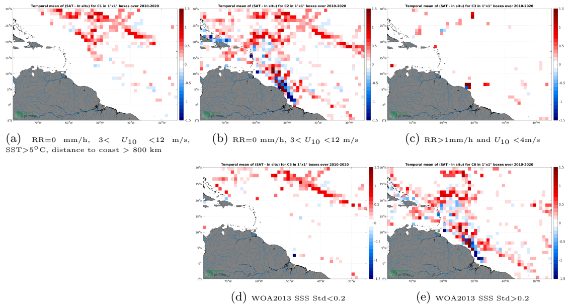
Figure 12: Temporal mean gridded over spatial boxes of size 1^\circ \times 1^\circ of \Delta SSS (CCI SSS L4 Merged-OI v3.2 - 7-day running (ESA) - TSG (SAMOS)) for 5 different subdatasets corresponding to:RR=0 mm/h, 3 < U_{10} < 12 m/s, SST >5^\circ\text{C} , distance to coast > 800 km (a), RR=0 mm/h, 3 < U_{10} < 12 m/s (b), RR >1 mm/h and U_{10} < 4 m/s (c), WOA2013 SSS Std <0.2 (d), WOA2013 SSS Std >0.2 (e).
