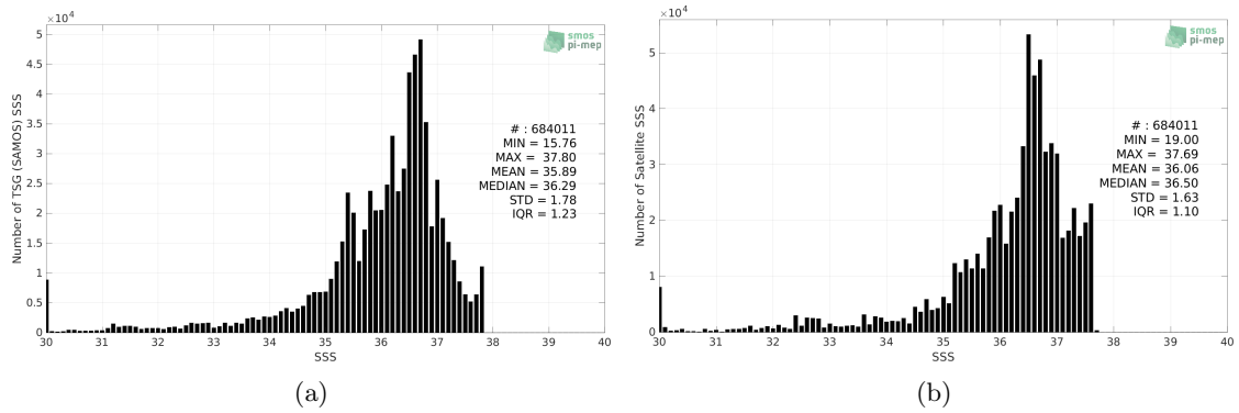
Figure 2: Histograms of SSS from TSG (SAMOS) (a) and CCI SSS L4 Merged-OI v3.2 - 7-day running (ESA) (b) considering all match-up pairs per bins of 0.1 over the Amazon and Orinoco river plumes Pi-MEP region and for the full satellite product period.
