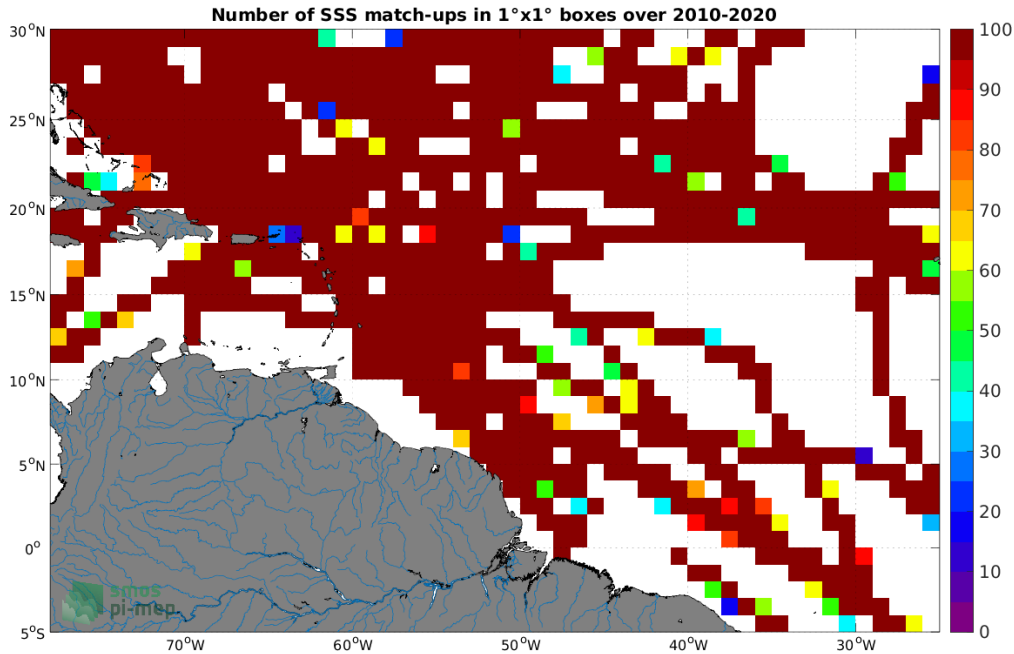
Figure 4: Number of SSS match-ups between TSG (SAMOS) SSS and the CCI SSS L4 Merged-OI v3.2 - 7-day running (ESA) SSS product for the Amazon and Orinoco river plumes Pi-MEP region over 1^\circ \times 1^\circ boxes and for the full satellite product period.
