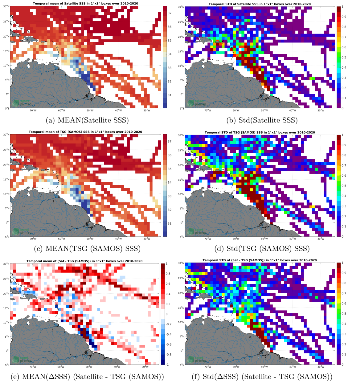
Figure 6: Temporal mean (left) and Std (right) of SSS from CCI SSS L4 Merged-OI v3.2 - 7-day running (ESA) (top), TSG (SAMOS) (middle), and of \Delta SSS (Satellite - TSG (SAMOS)). Only match-up pairs are used to generate these maps.
