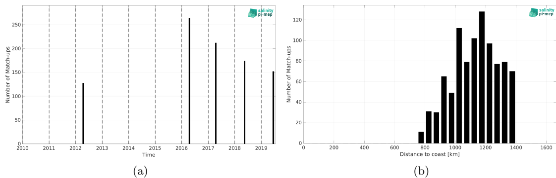
Figure 1: Number of match-ups between TSG (Polarstern) and CCI SSS L4 Merged-OI v3.2 - 7-day running (ESA) SSS as a function of time (a) and as function of the distance to coast (b) over the Amazon and Orinoco river plumes Pi-MEP region and for the full satellite product period.
