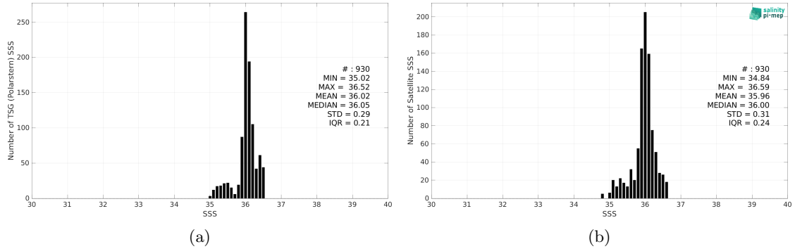
Figure 2: Histograms of SSS from TSG (Polarstern) (a) and CCI SSS L4 Merged-OI v3.2 - 7-day running (ESA) (b) considering all match-up pairs per bins of 0.1 over the Amazon and Orinoco river plumes Pi-MEP region and for the full satellite product period.
