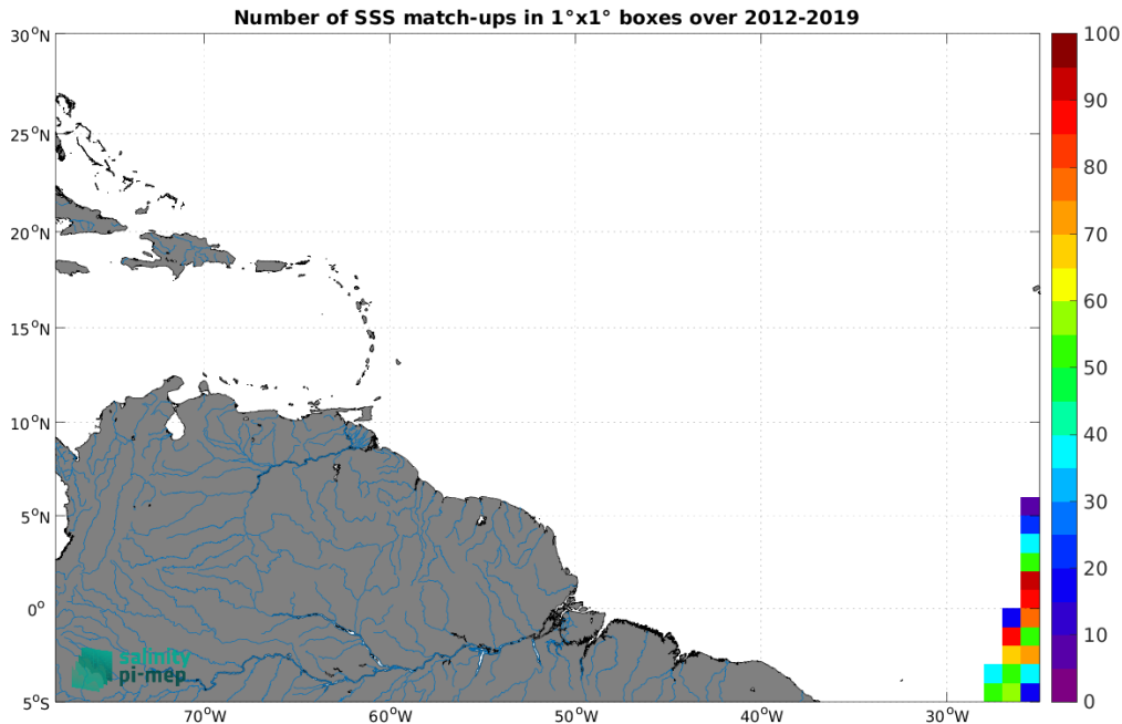
Figure 4: Number of SSS match-ups between TSG (Polarstern) SSS and the CCI SSS L4 Merged-OI v3.2 - 7-day running (ESA) SSS product for the Amazon and Orinoco river plumes Pi-MEP region over 1^\circ \times 1^\circ boxes and for the full satellite product period.
