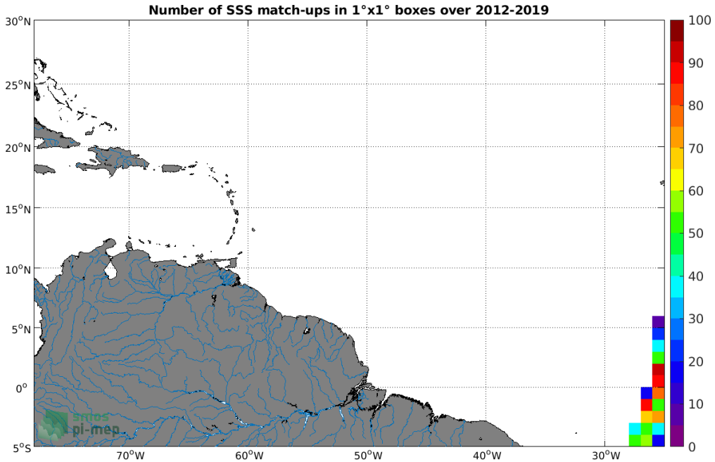
Figure 4: Number of SSS match-ups between TSG (Polarstern) SSS and the CCI SSS L4 Merged-OI v3.2 - 7-day running (ESA) SSS product for the Amazon and Orinoco river plumes Pi-MEP region over 1^{\circ} \times 1^{\circ} boxes and for the full satellite product period.
