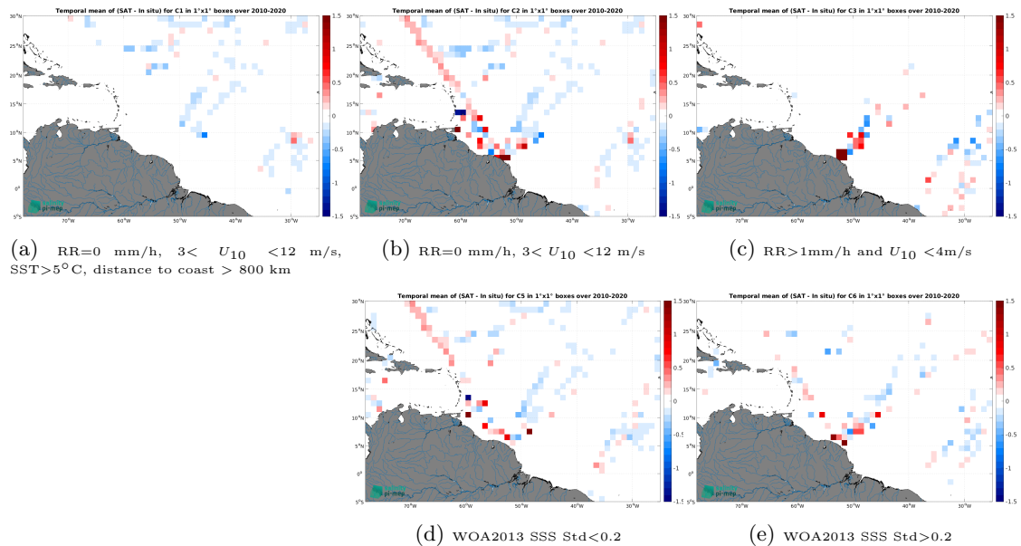
Figure 12: Temporal mean gridded over spatial boxes of size 1^\circ \times 1^\circ of \Delta\text{SSS} (CCI SSS L4 Merged-OI v3.2 - 7-day running (ESA) - TSG (LEGOS-DM)) for 5 different subdatasets corresponding to:RR=0 mm/h, 3 < U_{10} < 12 m/s, SST >5^\circ\text{C} , distance to coast > 800 km (a), RR=0 mm/h, 3 < U_{10} < 12 m/s (b), RR >1 mm/h and U_{10} < 4 m/s (c), WOA2013 SSS Std <0.2 (d), WOA2013 SSS Std >0.2 (e).
