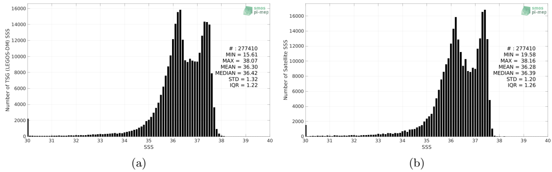
Figure 2: Histograms of SSS from TSG (LEGOS-DM) (a) and CCI SSS L4 Merged-OI v3.2 - 7-day running (ESA) (b) considering all match-up pairs per bins of 0.1 over the Amazon and Orinoco river plumes Pi-MEP region and for the full satellite product period.
