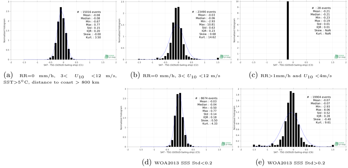
Figure 13: Normalized histogram of \Delta SSS (CCI SSS L4 Merged-OI v3.2 - 7-day running (ESA) - TSG (GOSUD-Sailing-ship)) for 5 different subdatasets corresponding to: RR=0 mm/h, 3 < U_{10} < 12 m/s, SST > 5°C, distance to coast > 800 km (a), RR=0 mm/h, 3 < U_{10} < 12 m/s (b), RR > 1mm/h and U_{10} < 4 m/s (c), WOA2013 SSS Std < 0.2 (d), WOA2013 SSS Std > 0.2 (e).
