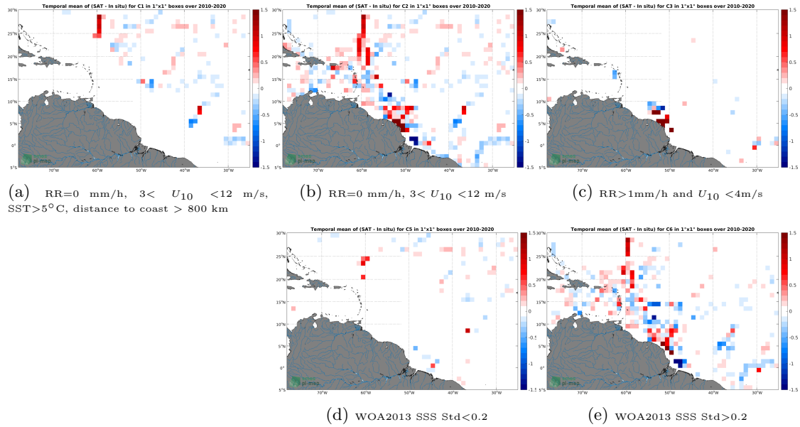
Figure 12: Temporal mean gridded over spatial boxes of size 1^\circ \times 1^\circ of \Delta SSS (CCI SSS L4 Merged-OI v3.2 - 7-day running (ESA) - TSG (GOSUD-Research-vessel)) for 5 different subdatasets corresponding to:RR=0 mm/h, 3 < U_{10} < 12 m/s, SST >5^\circ\text{C} , distance to coast > 800 km (a), RR=0 mm/h, 3 < U_{10} < 12 m/s (b), RR >1 mm/h and U_{10} < 4 m/s (c), WOA2013 SSS Std <0.2 (d), WOA2013 SSS Std >0.2 (e).
