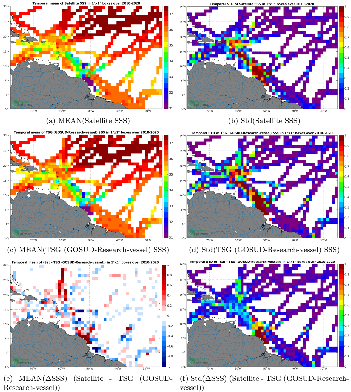
Figure 6: Temporal mean (left) and Std (right) of SSS from CCI SSS L4 Merged-OI v3.2 - 7-day running (ESA) (top), TSG (GOSUD-Research-vessel) (middle), and of \Delta SSS (Satellite - TSG (GOSUD-Research-vessel)). Only match-up pairs are used to generate these maps.
