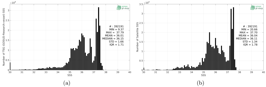
Figure 2: Histograms of SSS from TSG (GOSUD-Research-vessel) (a) and CCI SSS L4 Merged-OI v3.2 - 7-day running (ESA) (b) considering all match-up pairs per bins of 0.1 over the Amazon and Orinoco river plumes Pi-MEP region and for the full satellite product period.
