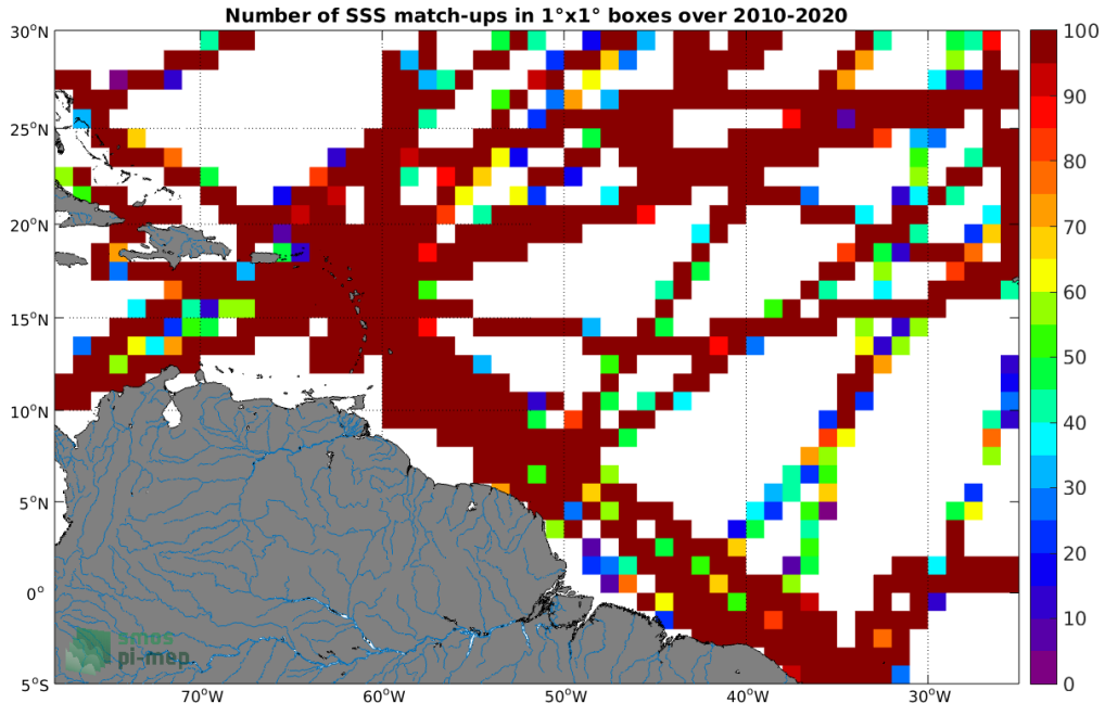
Figure 4: Number of SSS match-ups between TSG (GOSUD-Research-vessel) SSS and the CCI SSS L4 Merged-OI v3.2 - 7-day running (ESA) SSS product for the Amazon and Orinoco river plumes Pi-MEP region over 1^{\circ} \times 1^{\circ} boxes and for the full satellite product period.
