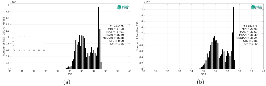
Figure 2: Histograms of SSS from TSG (CSIC-UTM) (a) and CCI SSS L4 Merged-OI v3.2 - 7-day running (ESA) (b) considering all match-up pairs per bins of 0.1 over the Amazon and Orinoco river plumes Pi-MEP region and for the full satellite product period.
