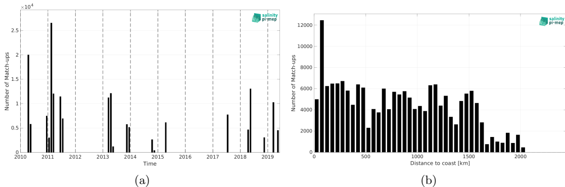
Figure 1: Number of match-ups between TSG (CSIC-UTM) and CCI SSS L4 Merged-OI v3.2 - 7-day running (ESA) SSS as a function of time (a) and as function of the distance to coast (b) over the Amazon and Orinoco river plumes Pi-MEP region and for the full satellite product period.
