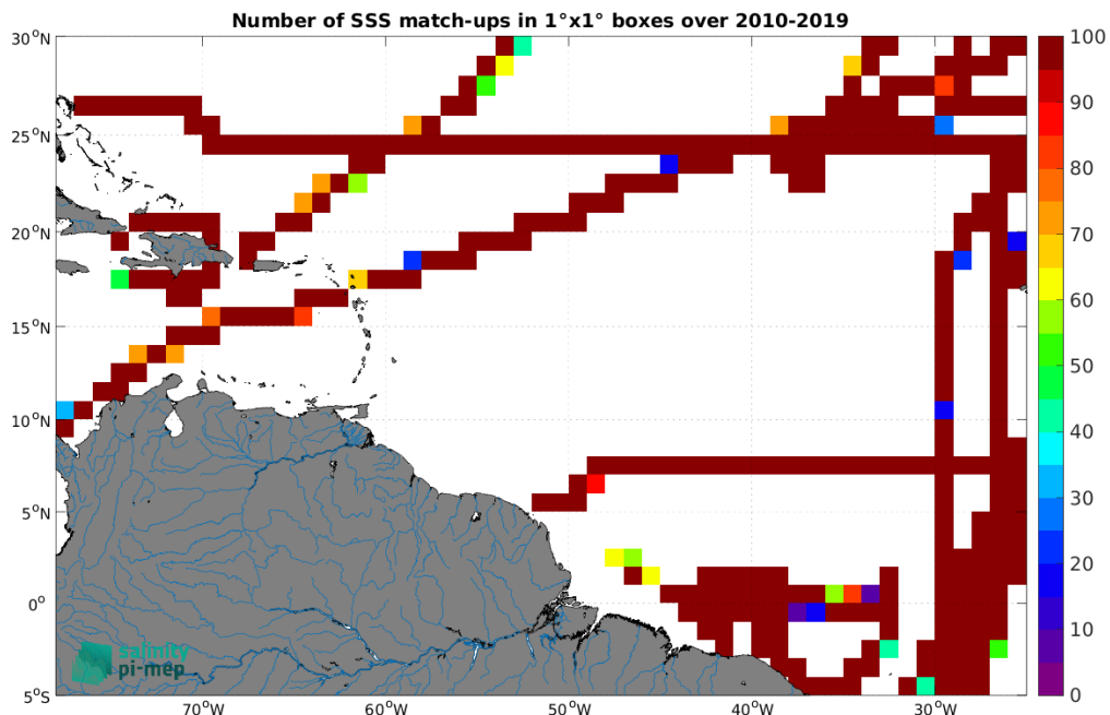
Figure 4: Number of SSS match-ups between TSG (CSIC-UTM) SSS and the CCI SSS L4 Merged-OI v3.2 - 7-day running (ESA) SSS product for the Amazon and Orinoco river plumes Pi-MEP region over 1^\circ \times 1^\circ boxes and for the full satellite product period.
