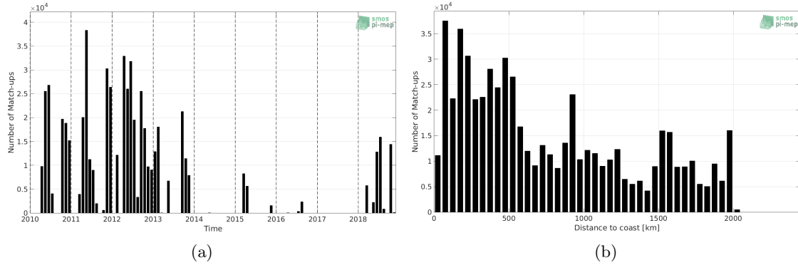
Figure 1: Number of match-ups between TSG-SAMOS and CCI L4 Merged-OI v1.8 - 7-day running (ESA) SSS as a function of time (a) and as function of the distance to coast (b) over the Amazon and Orinoco river plumes Pi-MEP region and for the full satellite product period.
