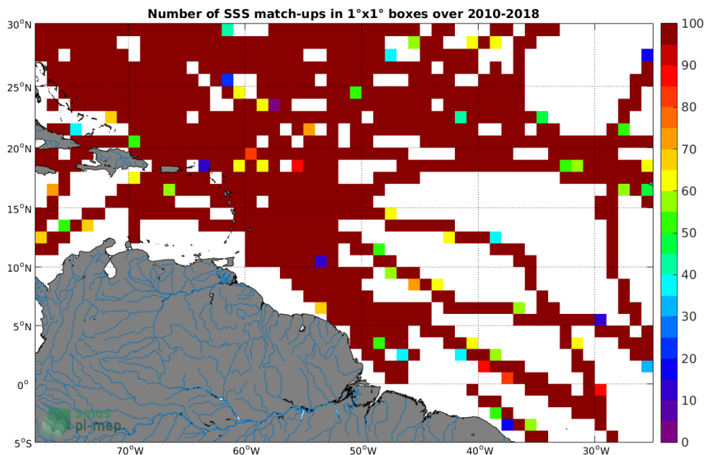
Figure 4: Number of SSS match-ups between TSG-SAMOS SSS and the CCI L4 Merged-OI v1.8 - 7-day running (ESA) SSS product for the Amazon and Orinoco river plumes Pi-MEP region over 1^\circ \times 1^\circ boxes and for the full satellite product period.
