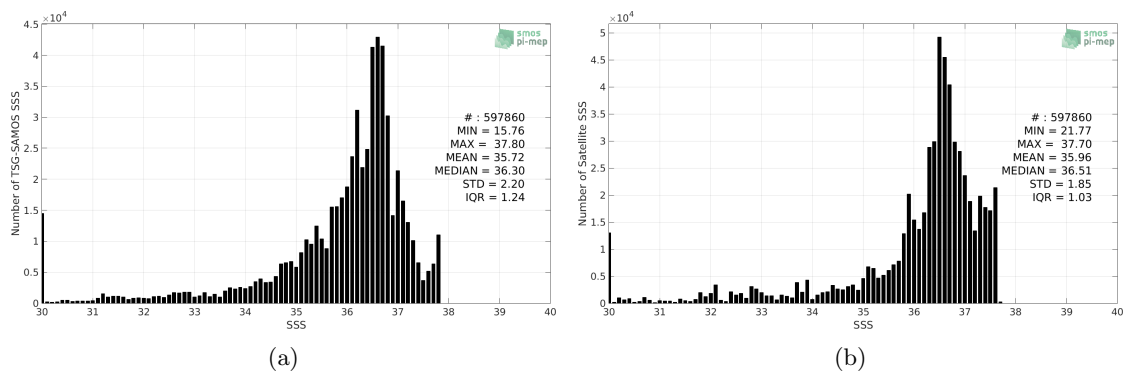
Figure 2: Histograms of SSS from TSG-SAMOS (a) and CCI L4 Merged-OI v1.8 - 7-day running (ESA) (b) considering all match-up pairs per bins of 0.1 over the Amazon and Orinoco river plumes Pi-MEP region and for the full satellite product period.
