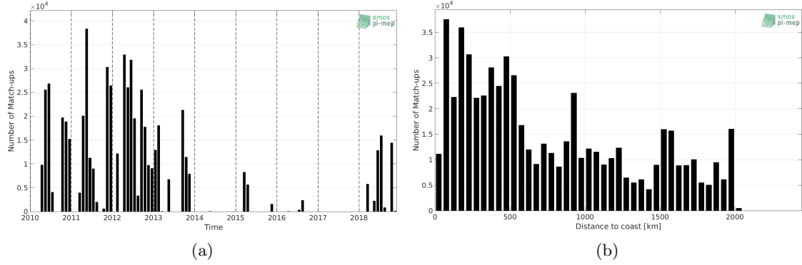
Figure 1: Number of match-ups between TSG-SAMOS and CCI-L4-ESA-MERGED-OI-V1.8-7DAY-RUNNING SSS as a function of time (a) and as function of the distance to coast (b) over the Amazon and Orinoco river plumes Pi-MEP region and for the full satellite product period.
