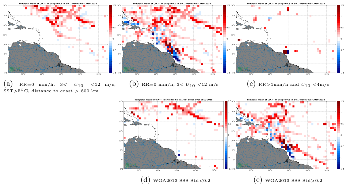
Figure 12: Temporal mean gridded over spatial boxes of size 1^\circ \times 1^\circ of \Delta SSS (CCI-L4-ESAMERGED-OI-V1.8-7DAY-RUNNING - TSG-SAMOS) for 5 different subdatasets corresponding to:RR=0 mm/h, 3 < U_{10} < 12 m/s, SST >5^\circ C, distance to coast > 800 km (a), RR=0 mm/h, 3 < U_{10} < 12 m/s (b), RR >1 mm/h and U_{10} < 4 m/s (c), WOA2013 SSS Std <0.2 (d), WOA2013 SSS Std >0.2 (e).
