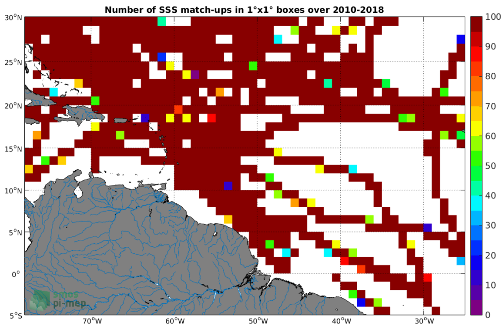
Figure 4: Number of SSS match-ups between TSG-SAMOS SSS and the CCI-L4-ESA-MERGED-OI-V1.8-7DAY-RUNNING SSS product for the Amazon and Orinoco river plumes Pi-MEP region over 1^\circ \times 1^\circ boxes and for the full satellite product period.
