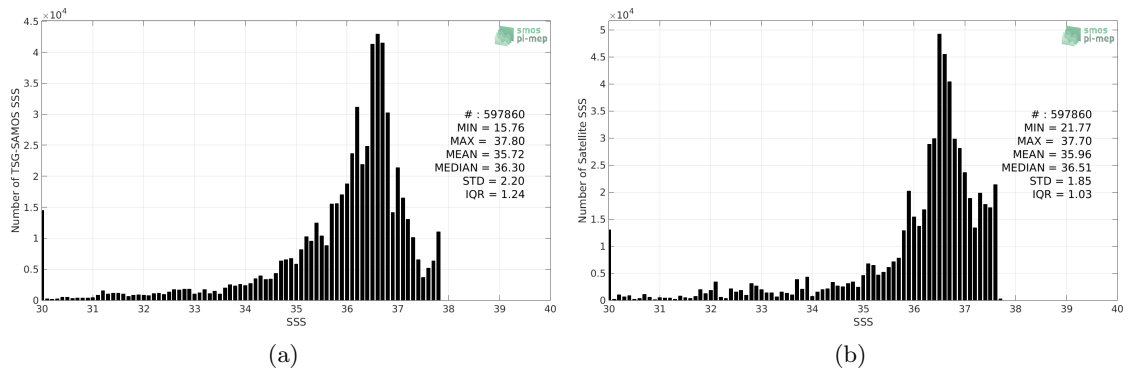
Figure 2: Histograms of SSS from TSG-SAMOS (a) and CCI-L4-ESA-MERGED-OI-V1.8-7DAY-RUNNING (b) considering all match-up pairs per bins of 0.1 over the Amazon and Orinoco river plumes Pi-MEP region and for the full satellite product period.
