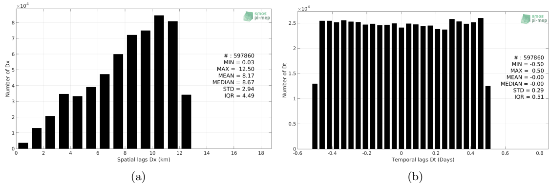
Figure 5: Histograms of the spatial (a) and temporal (b) lags between the time of the TSG-SAMOS measurements and the date of the corresponding CCI-L4-ESA-MERGED-OI-V1.8-7DAY-RUNNING SSS product.
