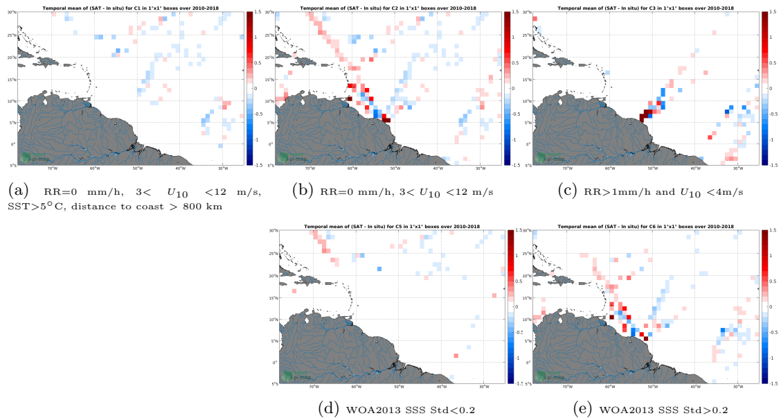
Figure 12: Temporal mean gridded over spatial boxes of size 1^\circ \times 1^\circ of \Delta SSS (CCI L4 Merged-OI v1.8 - 7-day running (ESA) - TSG-LEGOS-DM) for 5 different subdatasets corresponding to:RR=0 mm/h, 3 < U_{10} < 12 m/s, SST >5^\circ C, distance to coast > 800 km (a), RR=0 mm/h, 3 < U_{10} < 12 m/s (b), RR >1 mm/h and U_{10} < 4 m/s (c), WOA2013 SSS Std <0.2 (d), WOA2013 SSS Std >0.2 (e).
