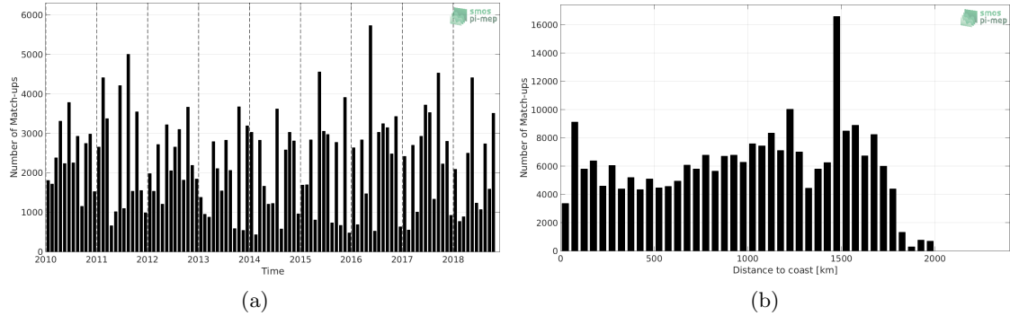
Figure 1: Number of match-ups between TSG-LEGOS-DM and CCI L4 Merged-OI v1.8 - 7-day running (ESA) SSS as a function of time (a) and as function of the distance to coast (b) over the Amazon and Orinoco river plumes Pi-MEP region and for the full satellite product period.
