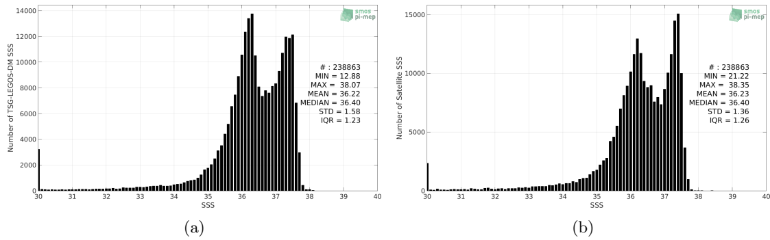
Figure 2: Histograms of SSS from TSG-LEGOS-DM (a) and CCI L4 Merged-OI v1.8 - 7-day running (ESA) (b) considering all match-up pairs per bins of 0.1 over the Amazon and Orinoco river plumes Pi-MEP region and for the full satellite product period.
