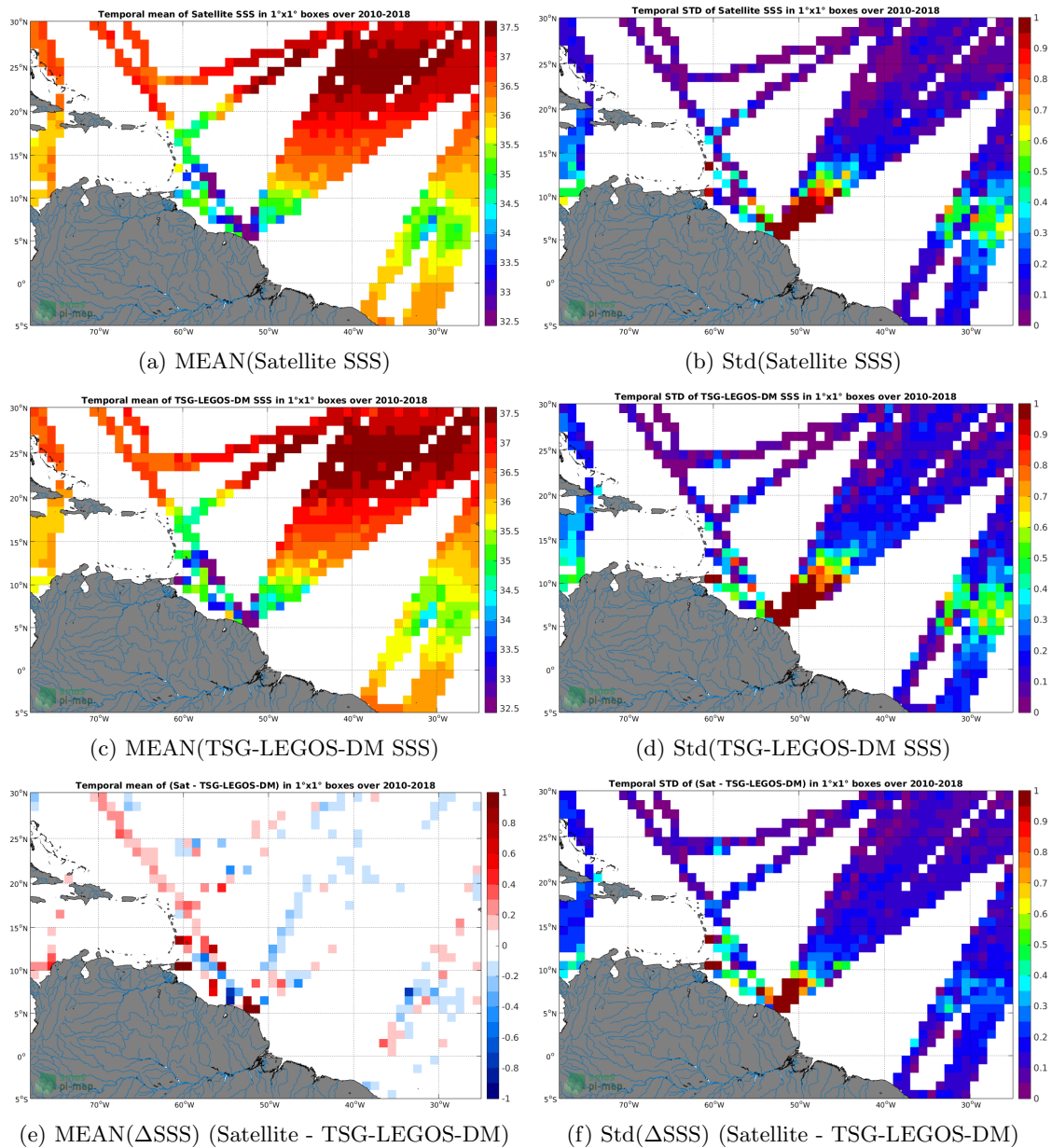
Figure 6: Temporal mean (left) and Std (right) of SSS from CCI L4 Merged-OI v1.8 - 7-day running (ESA) (top), TSG-LEGOS-DM (middle), and of \Delta SSS (Satellite - TSG-LEGOS-DM). Only match-up pairs are used to generate these maps.
