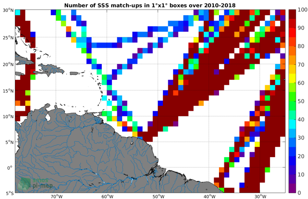
Figure 4: Number of SSS match-ups between TSG-LEGOS-DM SSS and the CCI L4 Merged-OI v1.8 - 7-day running (ESA) SSS product for the Amazon and Orinoco river plumes Pi-MEP region over 1^\circ \times 1^\circ boxes and for the full satellite product period.
