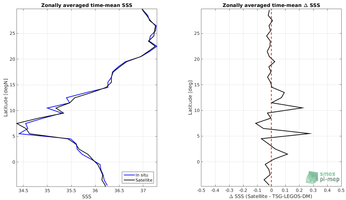
Figure 8: Left panel: Zonal mean SSS from CCI L4 Merged-OI v1.8 - 7-day running (ESA) satellite product (black) and from TSG-LEGOS-DM (blue). Right panel: Zonal mean of \Delta SSS (Satellite - TSG-LEGOS-DM) for all the collected Pi-MEP match-up pairs estimated over the full satellite product period.
