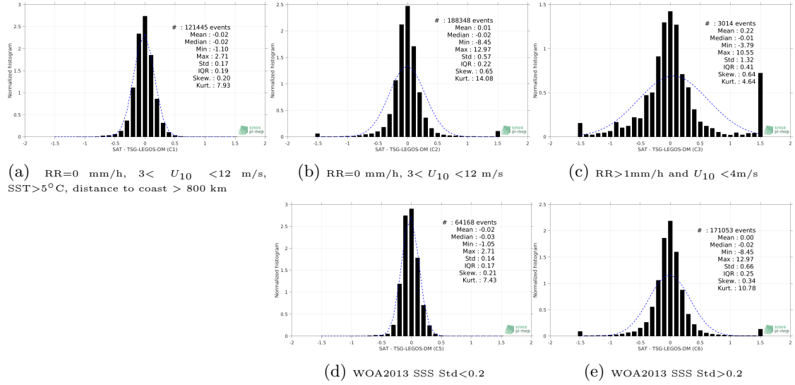
Figure 13: Normalized histogram of \Delta SSS (CCI L4 Merged-OI v1.8 - 7-day running (ESA) - TSG-LEGOS-DM) for 5 different subdatasets corresponding to: RR=0 mm/h, 3 < U_{10} < 12 m/s, SST>5°C, distance to coast > 800 km (a), RR=0 mm/h, 3 < U_{10} < 12 m/s (b), RR>1mm/h and U_{10} < 4 m/s (c), WOA2013 SSS Std<0.2 (d), WOA2013 SSS Std>0.2 (e).
