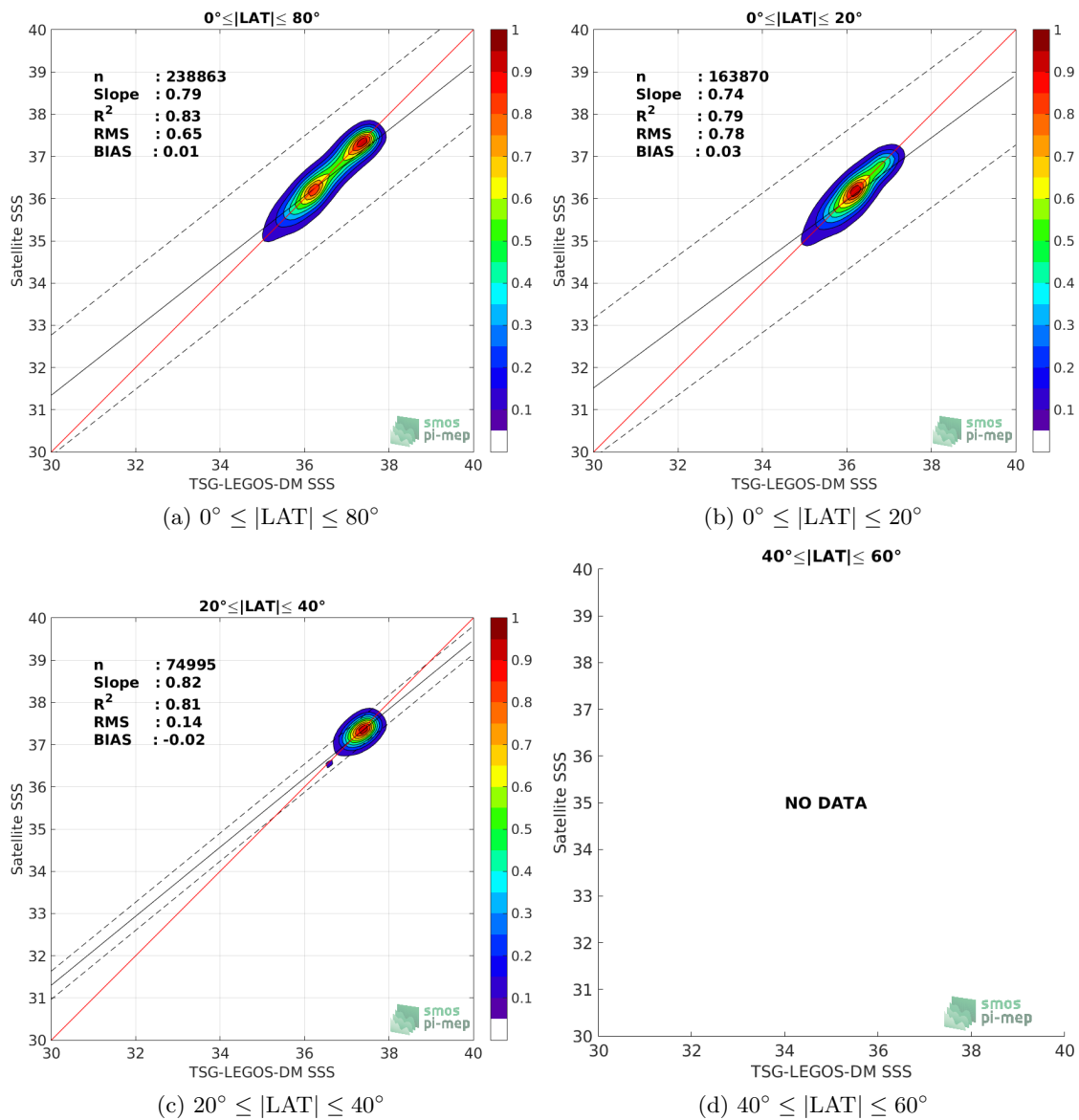
Figure 9: Contour maps of the concentration of CCI L4 Merged-OI v1.8 - 7-day running (ESA) SSS (y-axis) versus TSG-LEGOS-DM SSS (x-axis) at match-up pairs for different latitude bands. For each plot, the red line shows x=y . The black thin and dashed lines indicate a linear fit through the data cloud and the \pm 95\% confidence levels, respectively. The number match-up pairs n , the slope and R^2 coefficient of the linear fit, the root mean square (RMS) and the mean bias between satellite and in situ data are indicated for each latitude band in each plots.
