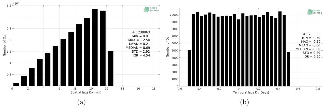
Figure 5: Histograms of the spatial (a) and temporal (b) lags between the time of the TSG-LEGOS-DM measurements and the date of the corresponding CCI L4 Merged-OI v1.8 - 7-day running (ESA) SSS product.
