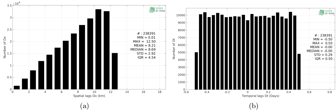
Figure 5: Histograms of the spatial (a) and temporal (b) lags between the time of the TSG-LEGOS-DM measurements and the date of the corresponding CCI-L4-ESA-MERGED-OI-V1.8-7DAY-RUNNING SSS product.
