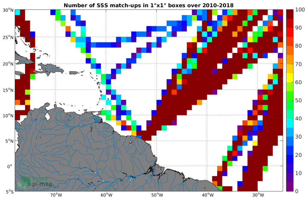
Figure 4: Number of SSS match-ups between TSG-LEGOS-DM SSS and the CCI-L4-ESA-MERGED-OI-V1.8-7DAY-RUNNING SSS product for the Amazon and Orinoco river plumes Pi-MEP region over 1^\circ \times 1^\circ boxes and for the full satellite product period.
