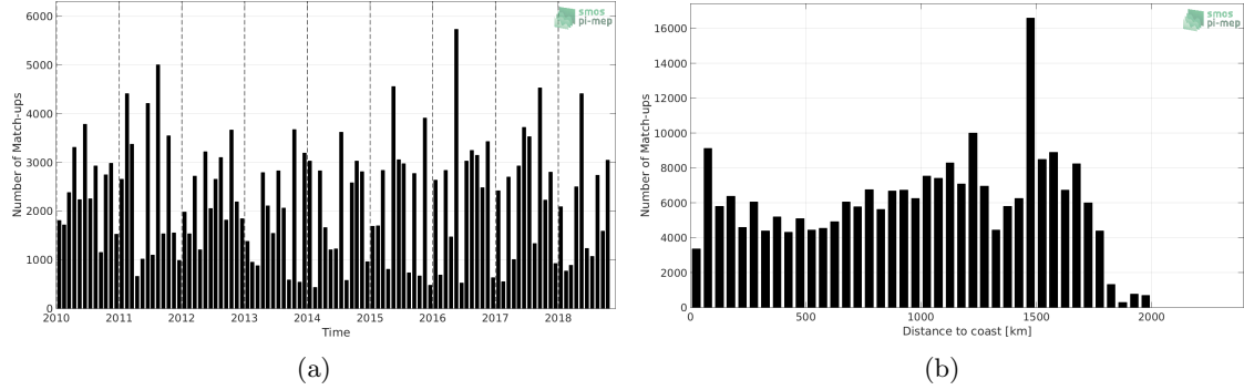
Figure 1: Number of match-ups between TSG-LEGOS-DM and CCI-L4-ESA-MERGED-OI-V1.8-7DAY-RUNNING SSS as a function of time (a) and as function of the distance to coast (b) over the Amazon and Orinoco river plumes Pi-MEP region and for the full satellite product period.
