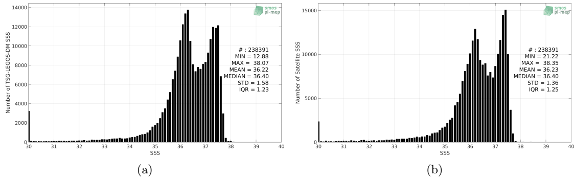
Figure 2: Histograms of SSS from TSG-LEGOS-DM (a) and CCI-L4-ESA-MERGED-OI-V1.8-7DAY-RUNNING (b) considering all match-up pairs per bins of 0.1 over the Amazon and Orinoco river plumes Pi-MEP region and for the full satellite product period.
