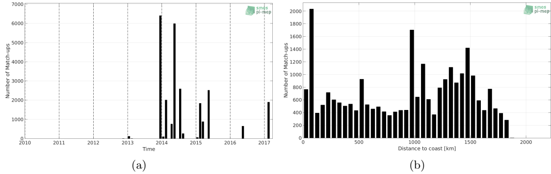
Figure 1: Number of match-ups between TSG-GOSUD-Sailing-ship and CCI L4 Merged-OI v1.8 - 7-day running (ESA) SSS as a function of time (a) and as function of the distance to coast (b) over the Amazon and Orinoco river plumes Pi-MEP region and for the full satellite product period.
