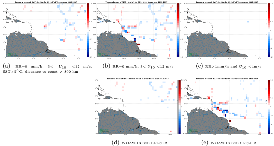
Figure 12: Temporal mean gridded over spatial boxes of size 1^{\circ}\times 1^{\circ} of \Delta SSS (CCI L4 Merged-OI v1.8 - 7-day running (ESA) - TSG-GOSUD-Sailing-ship) for 5 different subdatasets corresponding to:RR=0 mm/h, 3 < U_{10} < 12 m/s, SST >5^{\circ}\text{C} , distance to coast > 800 km (a), RR=0 mm/h, 3 < U_{10} < 12 m/s (b), RR >1 mm/h and U_{10} < 4 m/s (c), WOA2013 SSS Std <0.2 (d), WOA2013 SSS Std >0.2 (e).
