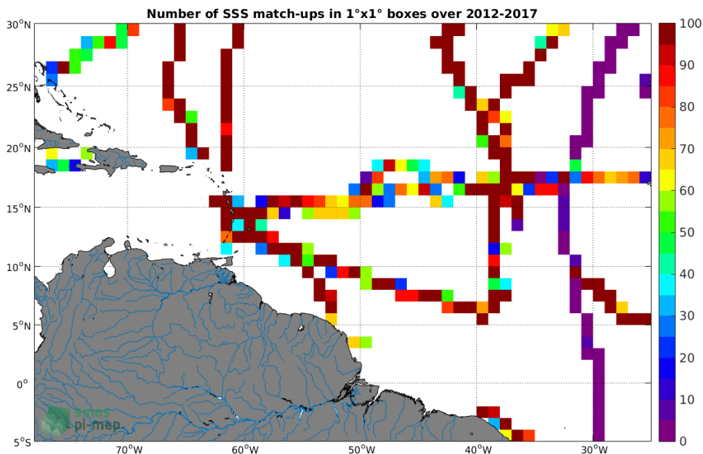
Figure 4: Number of SSS match-ups between TSG-GOSUD-Sailing-ship SSS and the CCI L4 Merged-OI v1.8 - 7-day running (ESA) SSS product for the Amazon and Orinoco river plumes Pi-MEP region over 1°x1° boxes and for the full satellite product period.
