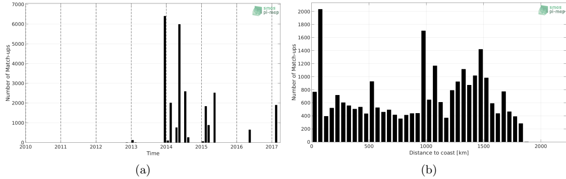
Figure 1: Number of match-ups between TSG-GOSUD-Sailing-ship and CCI-L4-ESA-MERGED-OI-V1.8-7DAY-RUNNING SSS as a function of time (a) and as function of the distance to coast (b) over the Amazon and Orinoco river plumes Pi-MEP region and for the full satellite product period.
