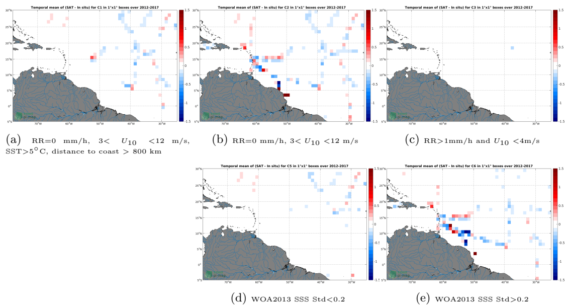
Figure 12: Temporal mean gridded over spatial boxes of size 1^\circ \times 1^\circ of \Delta SSS (CCI-L4-ESAMERGED-OI-V1.8-7DAY-RUNNING - TSG-GOSUD-Sailing-ship) for 5 different subdatasets corresponding to:RR=0 mm/h, 3 < U_{10} < 12 m/s, SST>5°C, distance to coast > 800 km (a), RR=0 mm/h, 3 < U_{10} < 12 m/s (b), RR>1mm/h and U_{10} < 4 m/s (c), WOA2013 SSS Std<0.2 (d), WOA2013 SSS Std>0.2 (e).
