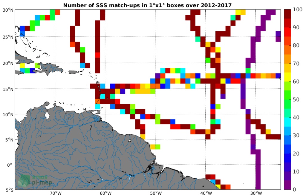
Figure 4: Number of SSS match-ups between TSG-GOSUD-Sailing-ship SSS and the CCI-L4-ESA-MERGED-OI-V1.8-7DAY-RUNNING SSS product for the Amazon and Orinoco river plumes Pi-MEP region over 1°x1° boxes and for the full satellite product period.
