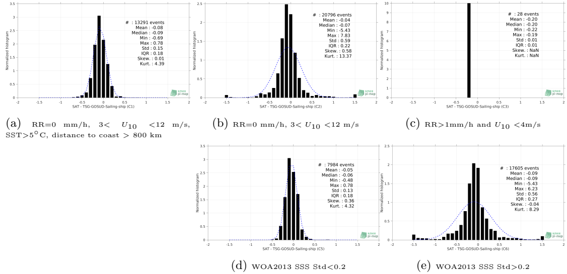
Figure 13: Normalized histogram of \Delta SSS (CCI-L4-ESA-MERGED-OI-V1.8-7DAY-RUNNING - TSG-GOSUD-Sailing-ship) for 5 different subdatasets corresponding to: RR=0 mm/h, 3 < U_{10} < 12 m/s, SST>5°C, distance to coast > 800 km (a), RR=0 mm/h, 3 < U_{10} < 12 m/s (b), RR>1mm/h and U_{10} < 4 m/s (c), WOA2013 SSS Std<0.2 (d), WOA2013 SSS Std>0.2 (e).
