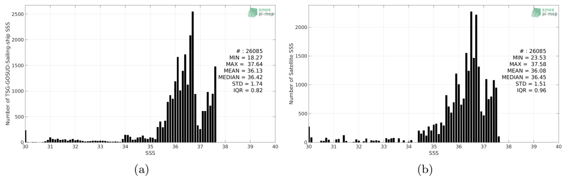
Figure 2: Histograms of SSS from TSG-GOSUD-Sailing-ship (a) and CCI-L4-ESA-MERGED-OI-V1.8-7DAY-RUNNING (b) considering all match-up pairs per bins of 0.1 over the Amazon and Orinoco river plumes Pi-MEP region and for the full satellite product period.
