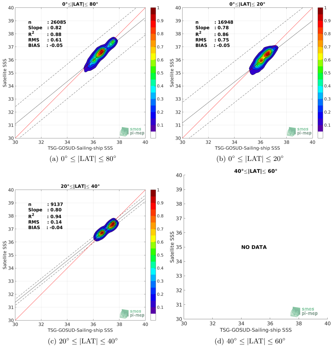
Figure 9: Contour maps of the concentration of CCI-L4-ESA-MERGED-OI-V1.8-7DAY-RUNNING SSS (y-axis) versus TSG-GOSUD-Sailing-ship SSS (x-axis) at match-up pairs for different latitude bands. For each plot, the red line shows x=y . The black thin and dashed lines indicate a linear fit through the data cloud and the \pm 95\% confidence levels, respectively. The number match-up pairs n , the slope and R^2 coefficient of the linear fit, the root mean square (RMS) and the mean bias between satellite and in situ data are indicated for each latitude band in each plots.
