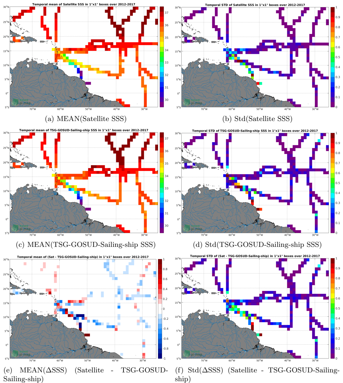
Figure 6: Temporal mean (left) and Std (right) of SSS from CCI-L4-ESA-MERGED-OI-V1.8-7DAY-RUNNING (top), TSG-GOSUD-Sailing-ship (middle), and of \Delta SSS (Satellite - TSG-GOSUD-Sailing-ship). Only match-up pairs are used to generate these maps.
