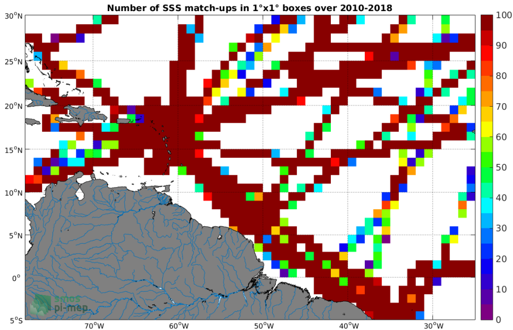
Figure 4: Number of SSS match-ups between TSG-GOSUD-Research-vessel SSS and the CCI L4 Merged-OI v1.8 - 7-day running (ESA) SSS product for the Amazon and Orinoco river plumes Pi-MEP region over 1°x1° boxes and for the full satellite product period.
