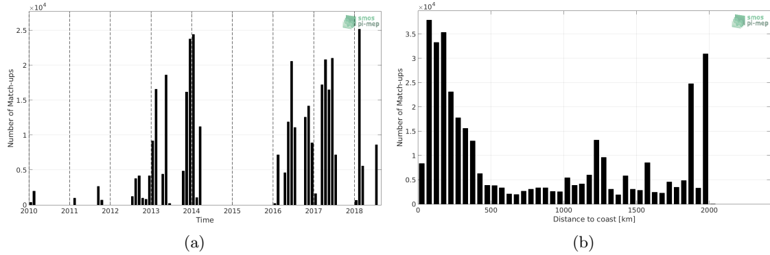
Figure 1: Number of match-ups between TSG-GOSUD-Research-vessel and CCI L4 Merged-OI v1.8 - 7-day running (ESA) SSS as a function of time (a) and as function of the distance to coast (b) over the Amazon and Orinoco river plumes Pi-MEP region and for the full satellite product period.
