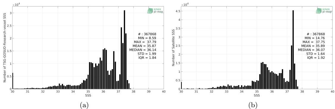
Figure 2: Histograms of SSS from TSG-GOSUD-Research-vessel (a) and CCI L4 Merged-OI v1.8 - 7-day running (ESA) (b) considering all match-up pairs per bins of 0.1 over the Amazon and Orinoco river plumes Pi-MEP region and for the full satellite product period.
