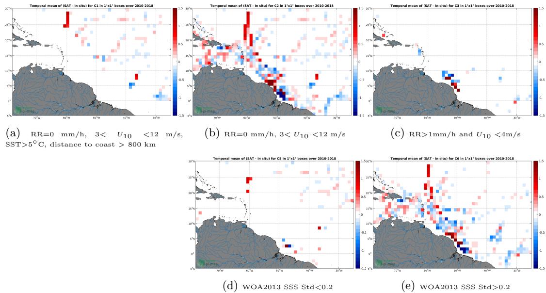
Figure 12: Temporal mean gridded over spatial boxes of size 1^{\circ}\times 1^{\circ} of \Delta SSS (CCI L4 Merged-OI v1.8 - 7-day running (ESA) - TSG-GOSUD-Research-vessel) for 5 different subdatasets corresponding to:RR=0 mm/h, 3 < U_{10} < 12 m/s, SST >5^{\circ}\text{C} , distance to coast > 800 km (a), RR=0 mm/h, 3 < U_{10} < 12 m/s (b), RR >1 mm/h and U_{10} < 4 m/s (c), WOA2013 SSS Std <0.2 (d), WOA2013 SSS Std >0.2 (e).
