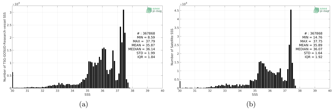
Figure 2: Histograms of SSS from TSG-GOSUD-Research-vessel (a) and CCI-L4-ESA-MERGED-OI-V1.8-7DAY-RUNNING (b) considering all match-up pairs per bins of 0.1 over the Amazon and Orinoco river plumes Pi-MEP region and for the full satellite product period.
