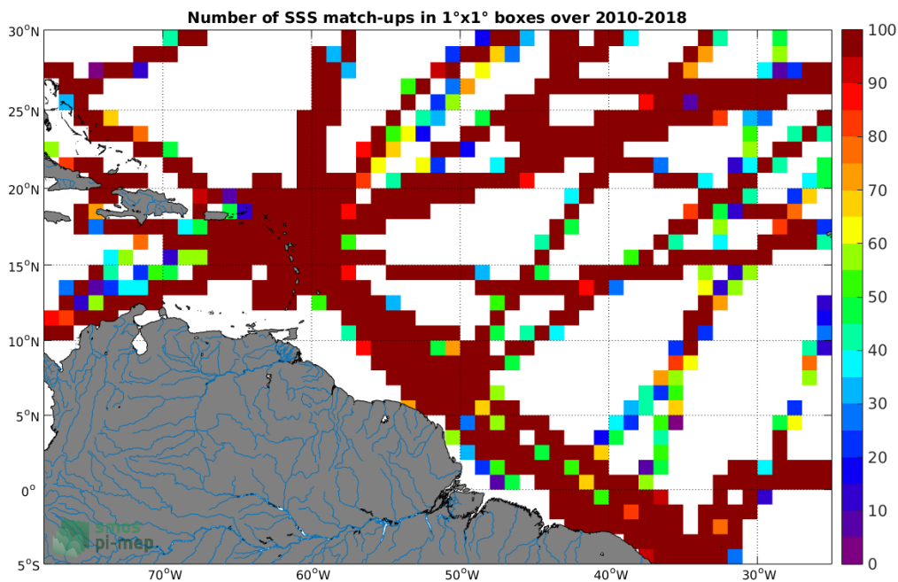
Figure 4: Number of SSS match-ups between TSG-GOSUD-Research-vessel SSS and the CCI-L4-ESA-MERGED-OI-V1.8-7DAY-RUNNING SSS product for the Amazon and Orinoco river plumes Pi-MEP region over 1°x1° boxes and for the full satellite product period.
