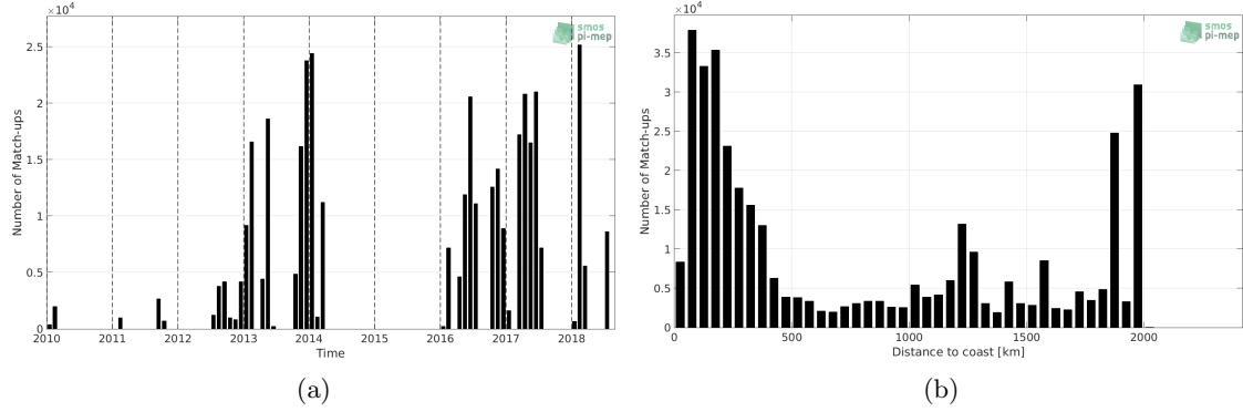
Figure 1: Number of match-ups between TSG-GOSUD-Research-vessel and CCI-L4-ESA-MERGED-OI-V1.8-7DAY-RUNNING SSS as a function of time (a) and as function of the distance to coast (b) over the Amazon and Orinoco river plumes Pi-MEP region and for the full satellite product period.
