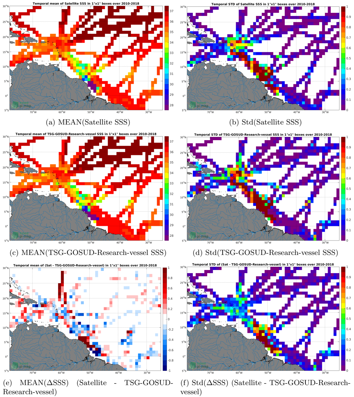
Figure 6: Temporal mean (left) and Std (right) of SSS from CCI-L4-ESA-MERGED-OI-V1.8-7DAY-RUNNING (top), TSG-GOSUD-Research-vessel (middle), and of \Delta SSS (Satellite - TSG-GOSUD-Research-vessel). Only match-up pairs are used to generate these maps.
