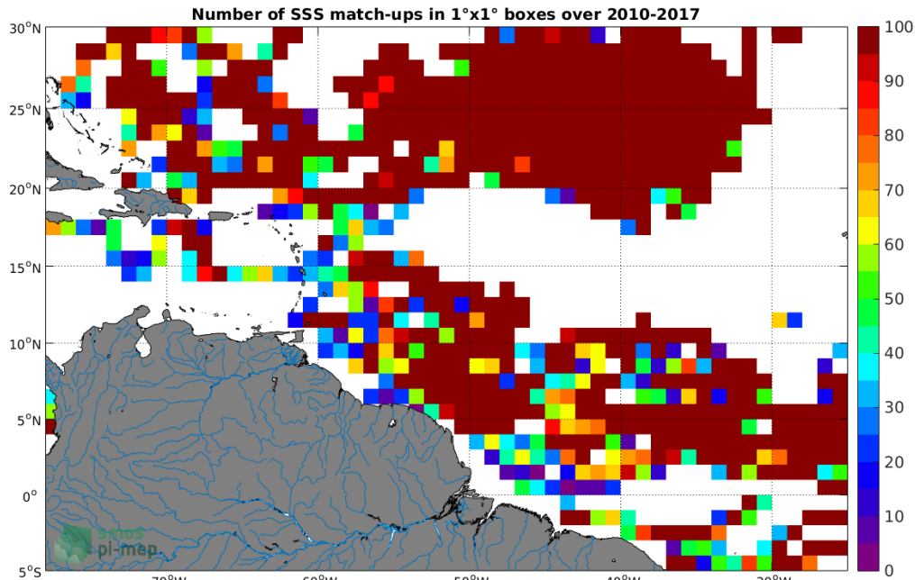
Figure 3: Number of SSS match-ups between Surface drifters SSS and the CCI L4 Merged-OI v1.8 - 7-day running (ESA) SSS product for the Amazon and Orinoco river plumes Pi-MEP region over 1°x1° boxes and for the full satellite product period.
