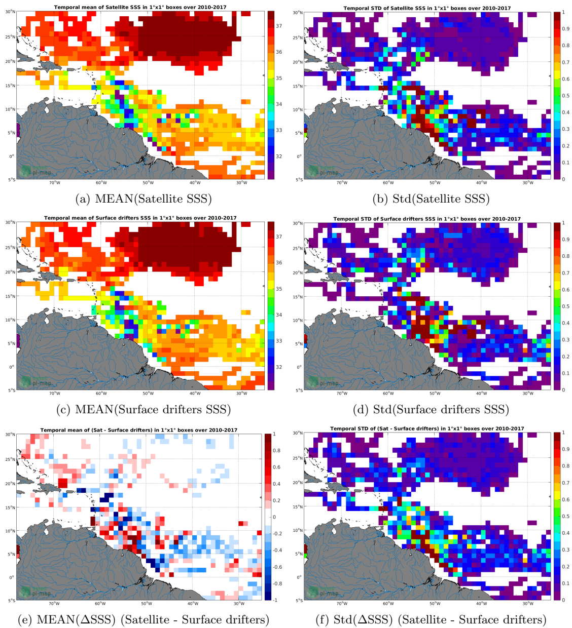
Figure 5: Temporal mean (left) and Std (right) of SSS from CCI L4 Merged-OI v1.8 - 7-day running (ESA) (top), Surface drifters (middle), and of \Delta SSS (Satellite - Surface drifters). Only match-up pairs are used to generate these maps.
