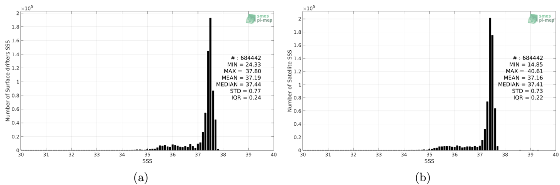
Figure 2: Histograms of SSS from Surface drifters (a) and CCI L4 Merged-OI v1.8 - 7-day running (ESA) (b) considering all match-up pairs per bins of 0.1 over the Amazon and Orinoco river plumes Pi-MEP region and for the full satellite product period.
