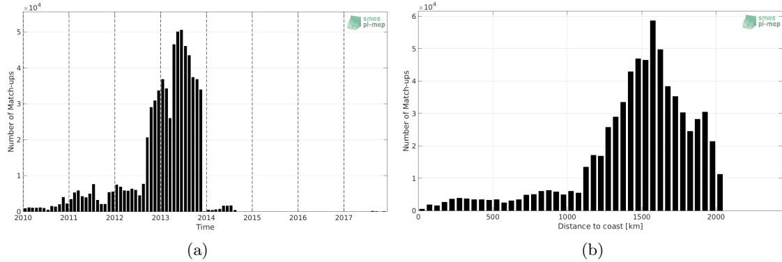
Figure 1: Number of match-ups between Surface drifters and CCI L4 Merged-OI v1.8 - 7-day running (ESA) SSS as a function of time (a) and as function of the distance to coast (b) over the Amazon and Orinoco river plumes Pi-MEP region and for the full satellite product period.
