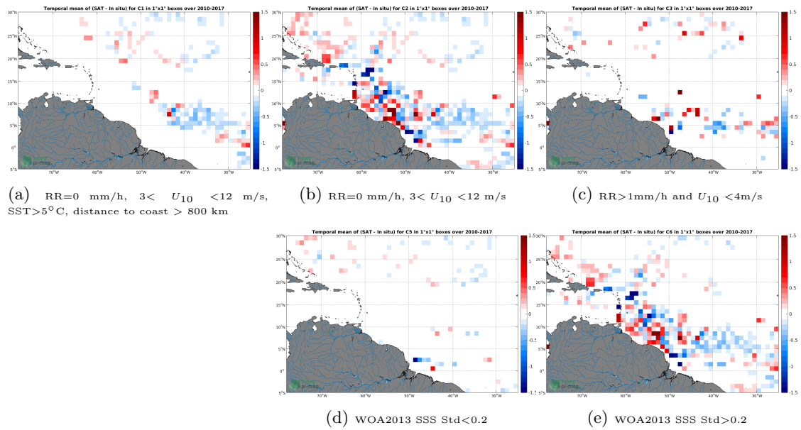
Figure 11: Temporal mean gridded over spatial boxes of size 1^\circ \times 1^\circ of \Delta SSS (CCI L4 Merged-OI v1.8 - 7-day running (ESA) - Surface drifters) for 5 different subdatasets corresponding to:RR=0 mm/h, 3 < U_{10} < 12 m/s, SST >5^\circ\text{C} , distance to coast > 800 km (a), RR=0 mm/h, 3 < U_{10} < 12 m/s (b), RR >1 mm/h and U_{10} < 4 m/s (c), WOA2013 SSS Std <0.2 (d), WOA2013 SSS Std >0.2 (e).
