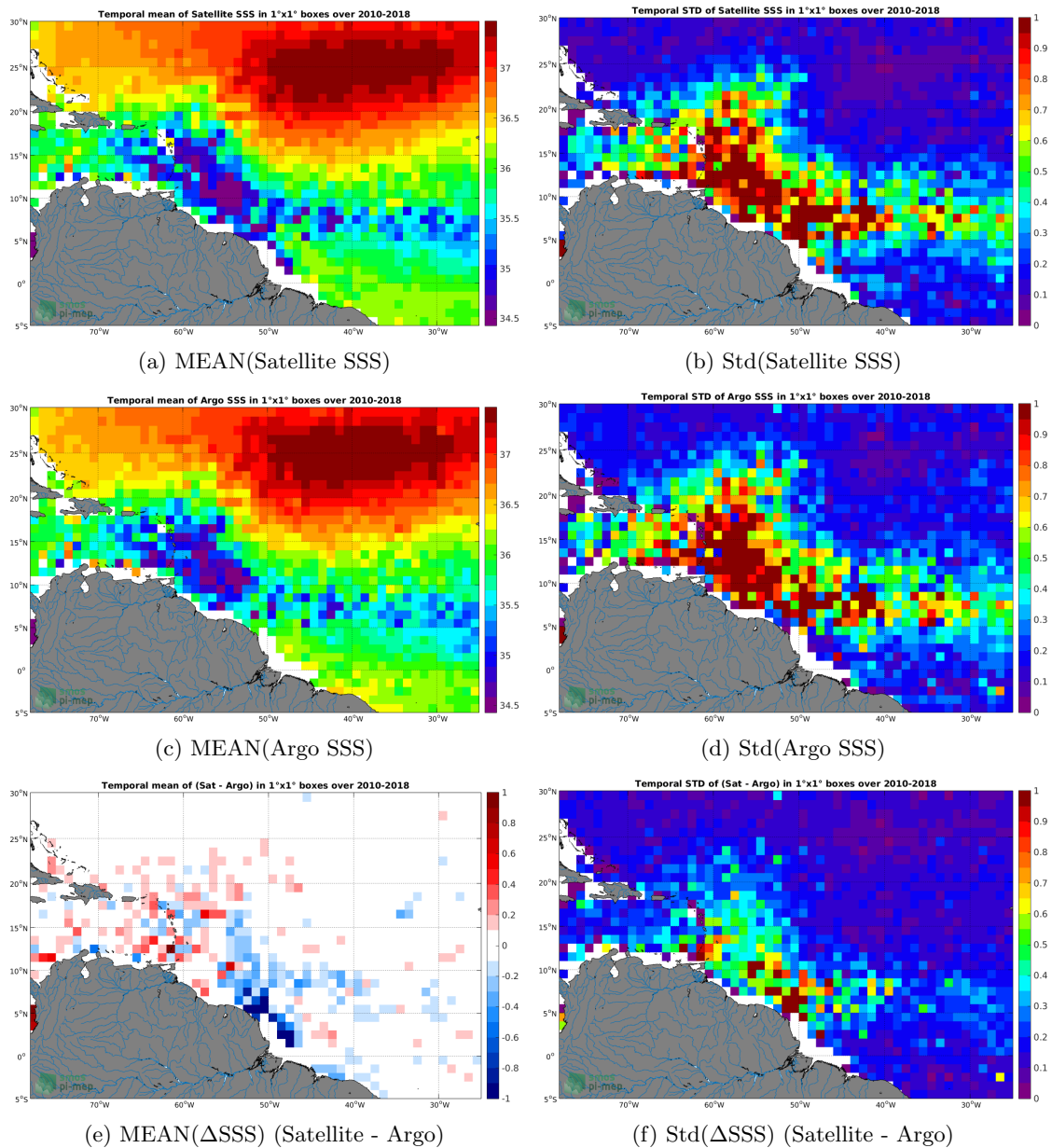
Figure 6: Temporal mean (left) and Std (right) of SSS from CCI-L4-ESA-MERGED-OI-V1.8-7DAY-RUNNING (top), Argo (middle), and of \Delta SSS (Satellite - Argo). Only match-up pairs are used to generate these maps.
