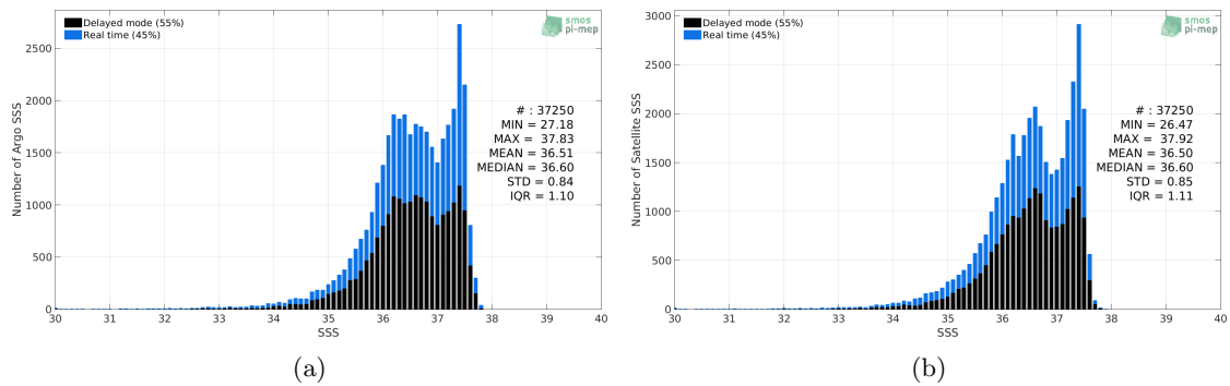
Figure 2: Histograms of SSS from Argo (a) and CCI-L4-ESA-MERGED-OI-V1.8-7DAY-RUNNING (b) considering all match-up pairs per bins of 0.1 over the Amazon and Orinoco river plumes Pi-MEP region and for the full satellite product period.
