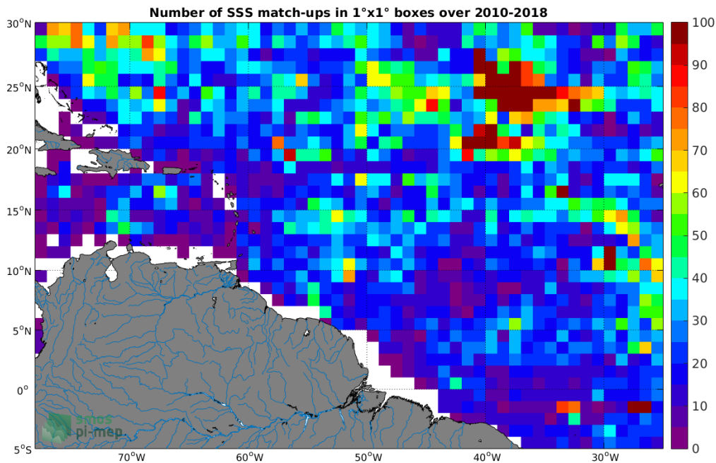
Figure 4: Number of SSS match-ups between Argo SSS and the CCI-L4-ESA-MERGED-OI-V1.8-7DAY-RUNNING SSS product for the Amazon and Orinoco river plumes Pi-MEP region over 1°x1° boxes and for the full satellite product period.
