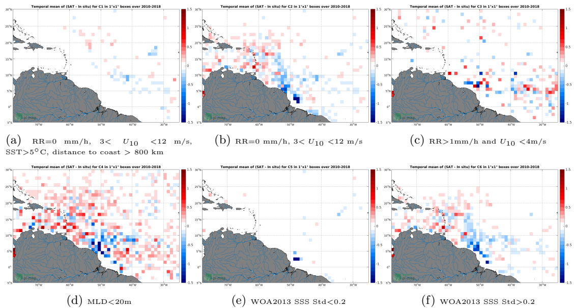
Figure 12: Temporal mean gridded over spatial boxes of size 1^\circ \times 1^\circ of \Delta SSS (CCI-L4-ESA-MERGED-OI-V1.8-7DAY-RUNNING - Argo) for 6 different subdatasets corresponding to:RR=0 mm/h, 3 < U_{10} < 12 m/s, SST >5^\circ C, distance to coast > 800 km (a), RR=0 mm/h, 3 < U_{10} < 12 m/s (b), RR >1 mm/h and U_{10} < 4 m/s (c),MLD <20 m (d),WOA2013 SSS Std <0.2 (e),WOA2013 SSS Std >0.2 (f).
