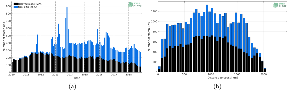
Figure 1: Number of match-ups between Argo and CCI-L4-ESA-MERGED-OI-V1.8-7DAY-RUNNING SSS as a function of time (a) and as function of the distance to coast (b) over the Amazon and Orinoco river plumes Pi-MEP region and for the full satellite product period.
