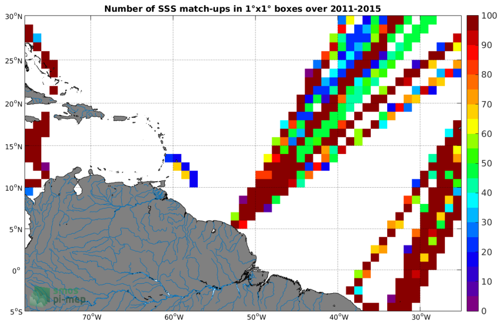
Figure 4: Number of SSS match-ups between TSG-LEGOS-DM SSS and the Aquarius-L4-IPRC-V5-WEEKLY SSS product for the Amazon and Orinoco river plumes Pi-MEP region over 1^\circ \times 1^\circ boxes and for the full satellite product period.
