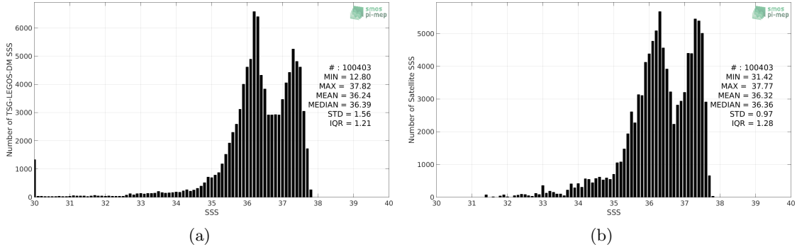
Figure 2: Histograms of SSS from TSG-LEGOS-DM (a) and Aquarius-L4-IPRC-V5-WEEKLY (b) considering all match-up pairs per bins of 0.1 over the Amazon and Orinoco river plumes Pi-MEP region and for the full satellite product period.
