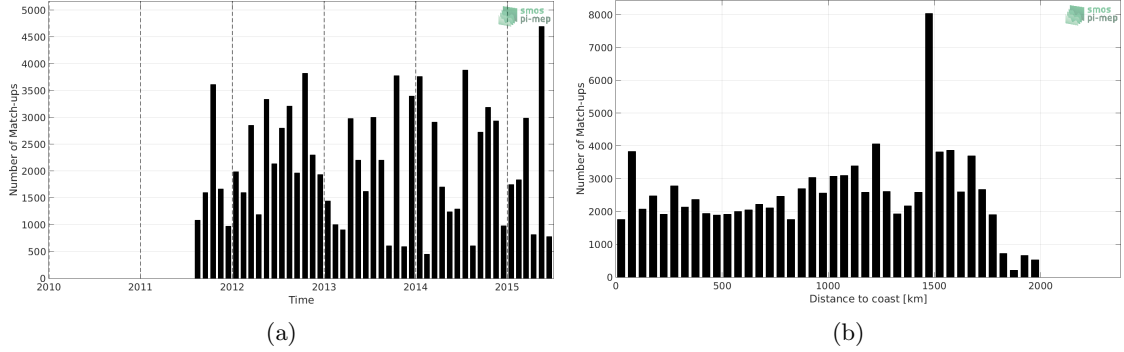
Figure 1: Number of match-ups between TSG-LEGOS-DM and Aquarius-L4-IPRC-V5-WEEKLY SSS as a function of time (a) and as function of the distance to coast (b) over the Amazon and Orinoco river plumes Pi-MEP region and for the full satellite product period.
