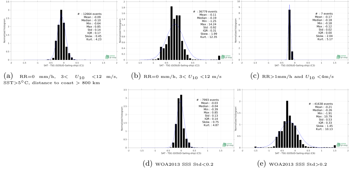
Figure 13: Normalized histogram of \Delta SSS (Aquarius SSS L4 OI v5 - Weekly (IPRC) - TSG (GOSUD-Sailing-ship)) for 5 different subdatasets corresponding to: RR=0 mm/h, 3 < U_{10} < 12 m/s, SST > 5^\circ\text{C} , distance to coast > 800 km (a), RR=0 mm/h, 3 < U_{10} < 12 m/s (b), RR > 1 mm/h and U_{10} < 4 m/s (c), WOA2013 SSS Std < 0.2 (d), WOA2013 SSS Std > 0.2 (e).
