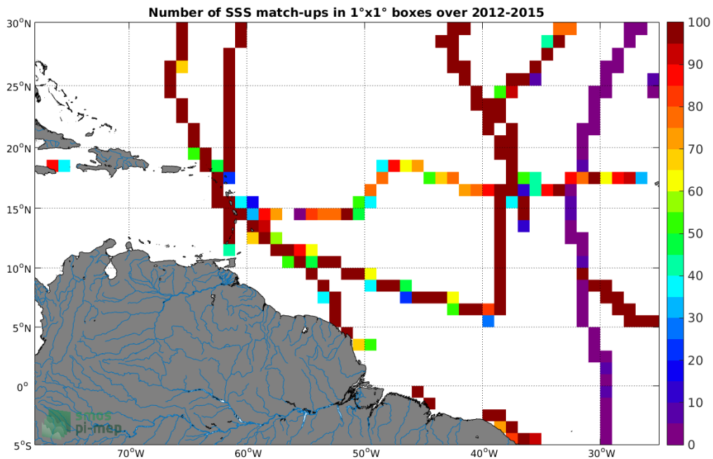
Figure 4: Number of SSS match-ups between TSG-GOSUD-Sailing-ship SSS and the Aquarius-L4-IPRC-V5-WEEKLY SSS product for the Amazon and Orinoco river plumes Pi-MEP region over 1°x1° boxes and for the full satellite product period.
