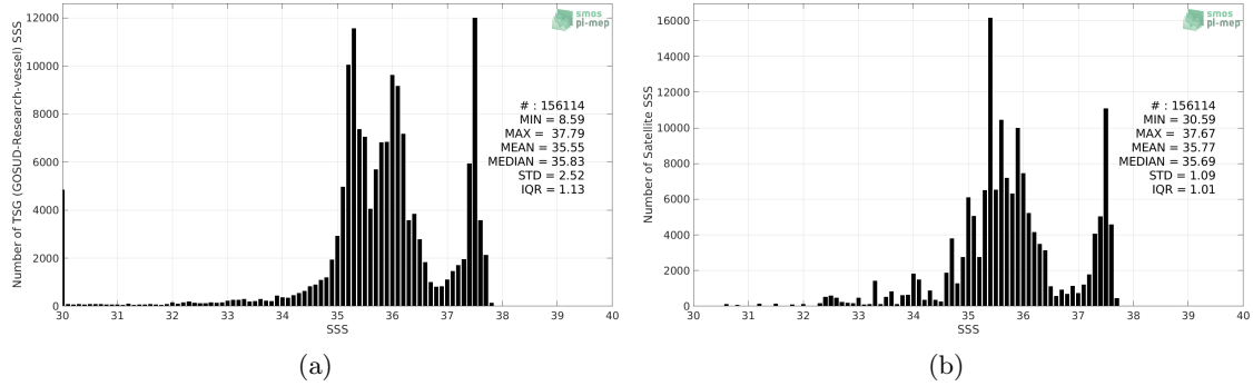
Figure 2: Histograms of SSS from TSG (GOSUD-Research-vessel) (a) and Aquarius SSS L4 OI v5 - Weekly (IPRC) (b) considering all match-up pairs per bins of 0.1 over the Amazon and Orinoco river plumes Pi-MEP region and for the full satellite product period.
