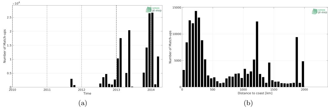
Figure 1: Number of match-ups between TSG (GOSUD-Research-vessel) and Aquarius SSS L4 OI v5 - Weekly (IPRC) SSS as a function of time (a) and as function of the distance to coast (b) over the Amazon and Orinoco river plumes Pi-MEP region and for the full satellite product period.
