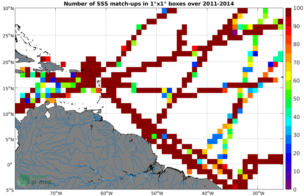
Figure 4: Number of SSS match-ups between TSG (GOSUD-Research-vessel) SSS and the Aquarius SSS L4 OI v5 - Weekly (IPRC) SSS product for the Amazon and Orinoco river plumes Pi-MEP region over 1^\circ \times 1^\circ boxes and for the full satellite product period.
